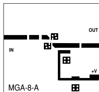
Figure 14. PCB Layout.
