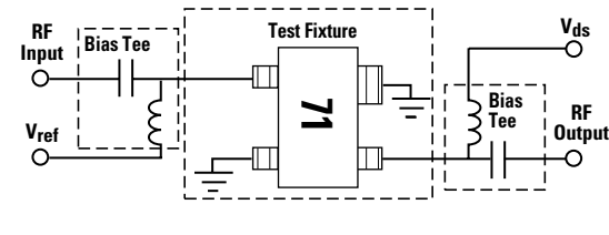
Figure 5. MGA-71543 Test Circuit for S, Noise, and Power Parameters over Frequency.
