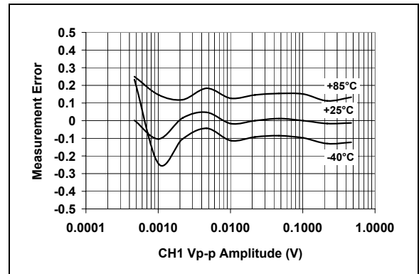
FIGURE 2-10: Measurement Error, Gain = 2, PF = + 0.5.
