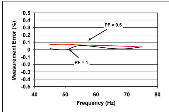
FIGURE 2-11: Measurement Error vs. Input Frequency.
