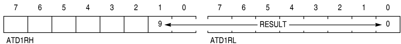
Figure 14-8. Right-Justified Mode
