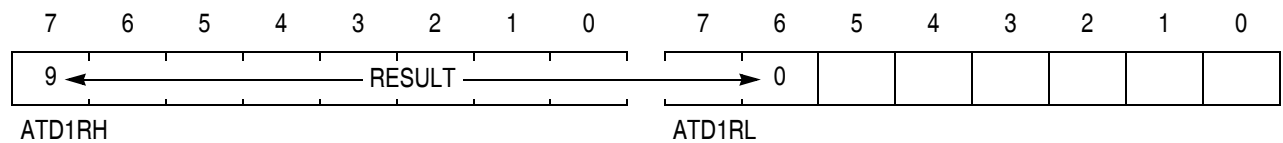
Figure 14-7. Left-Justified Mode
