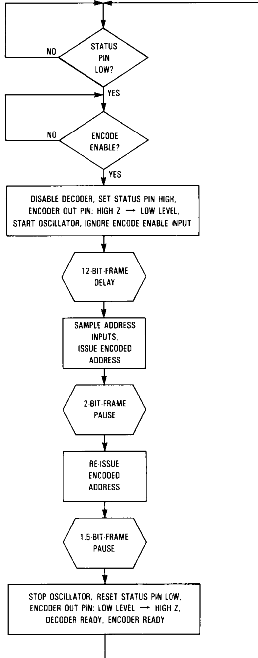
Figure 8. Encoder Flowchart
