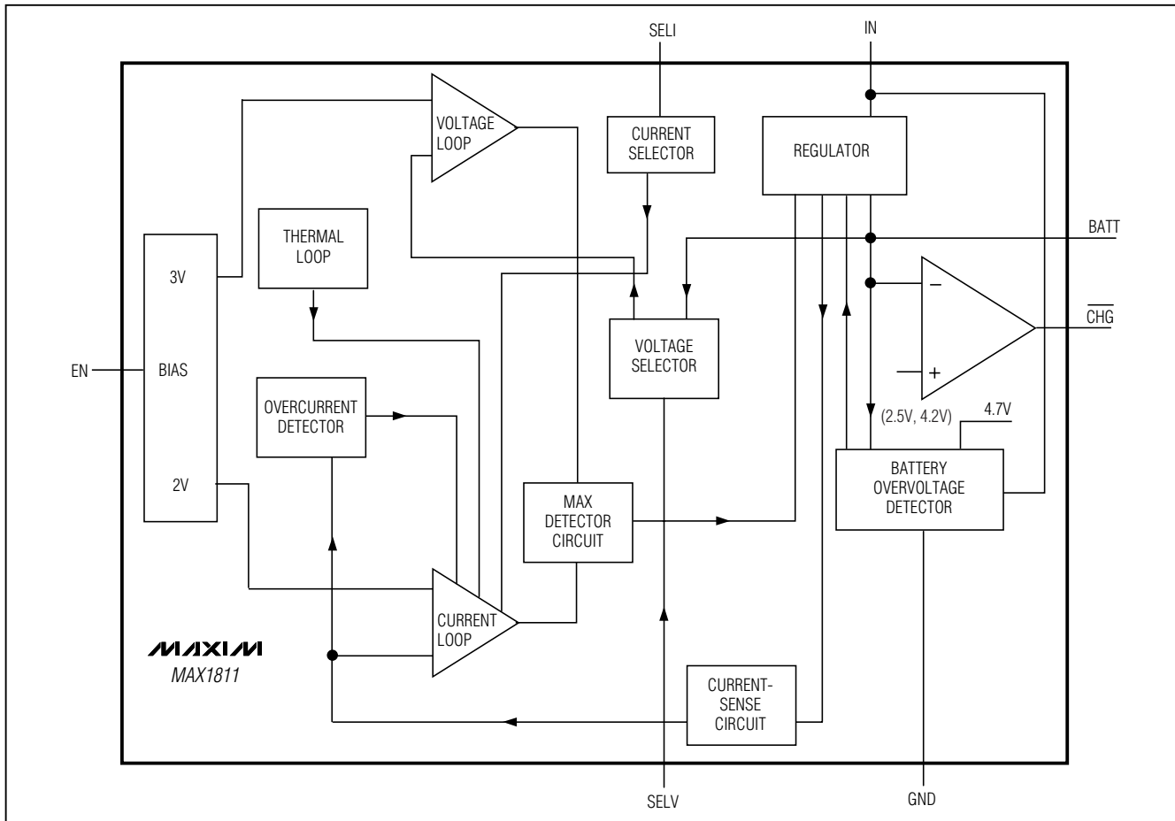
Figure 1. Functional Diagram
