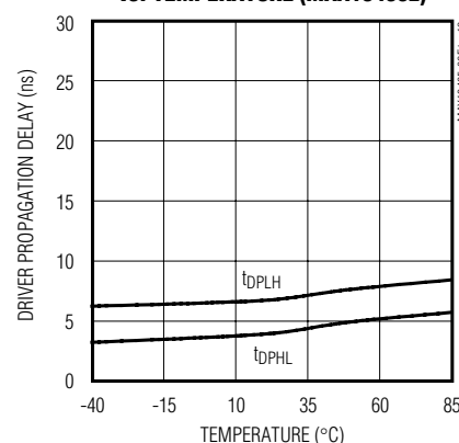
DRIVER PROPAGATION DELAY vs. TEMPERATURE (MAX13486E)
