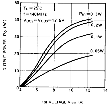
OUTPUT POWER VS. 1st VOLTAGE (M57729)
