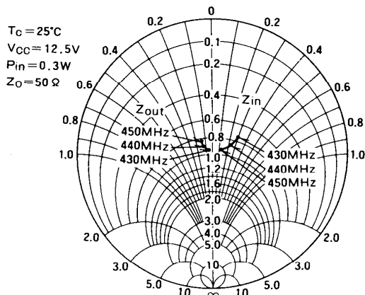
INPUT IMPEDANCE, OUTPUT IMPEDANCE VS. FREQUENCY (M57729)
