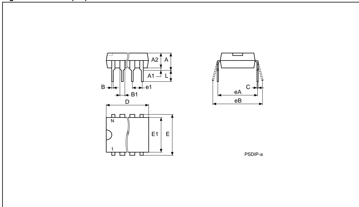
Figure 16. PSDIP8 (BN)
