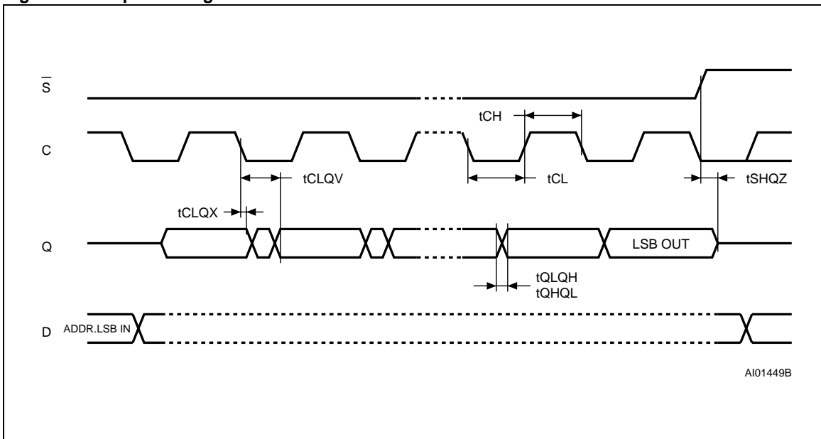
Figure 15. Output Timing
