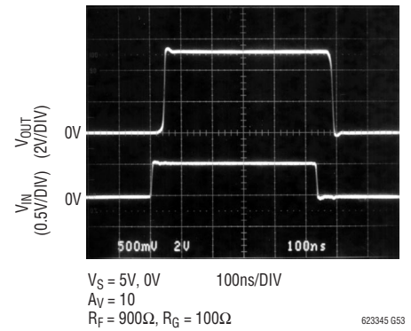
Output-Overload Recovery
