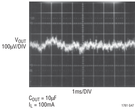
LT1761-5 10Hz to 100kHz Output Noise C_{BYYP} = 1000\text{pF}
