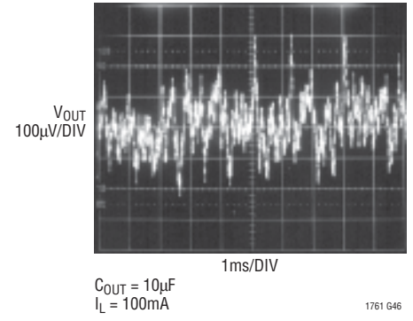
LT1761-5 10Hz to 100kHz Output Noise C_{BYYP} = 100\text{pF}
