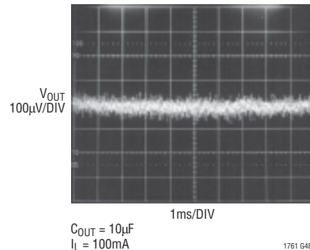
LT1761-5 10Hz to 100kHz Output Noise C_{BYYP} = 0.01\mu\text{F}
