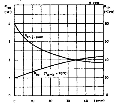
Figure 33. Maximum dissipable power and junction to ambient thermal resistance vs. side "l"
