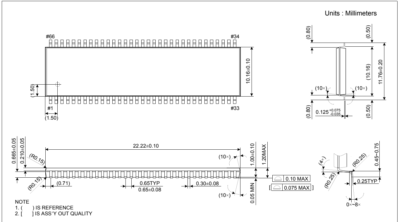
66pin TSOP II / Package dimension
