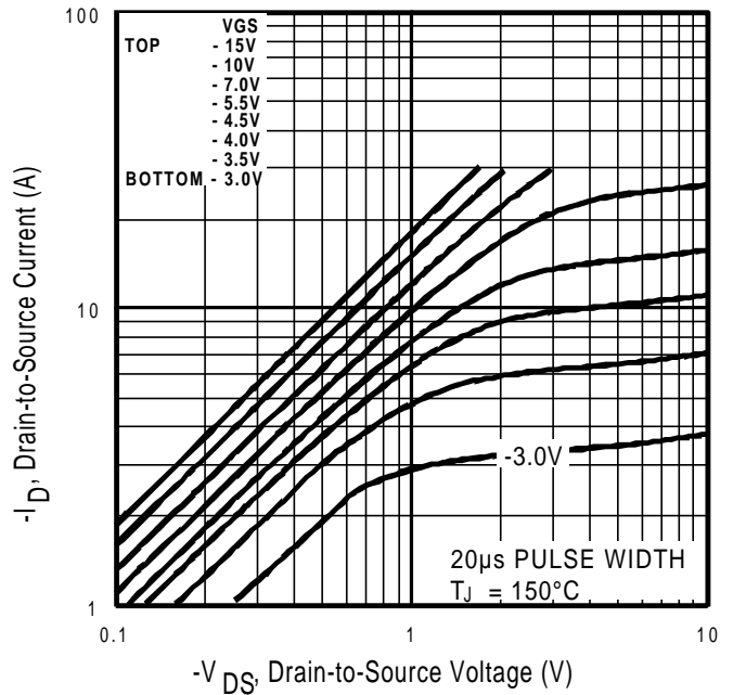
Fig 13. Typical Output Characteristics
