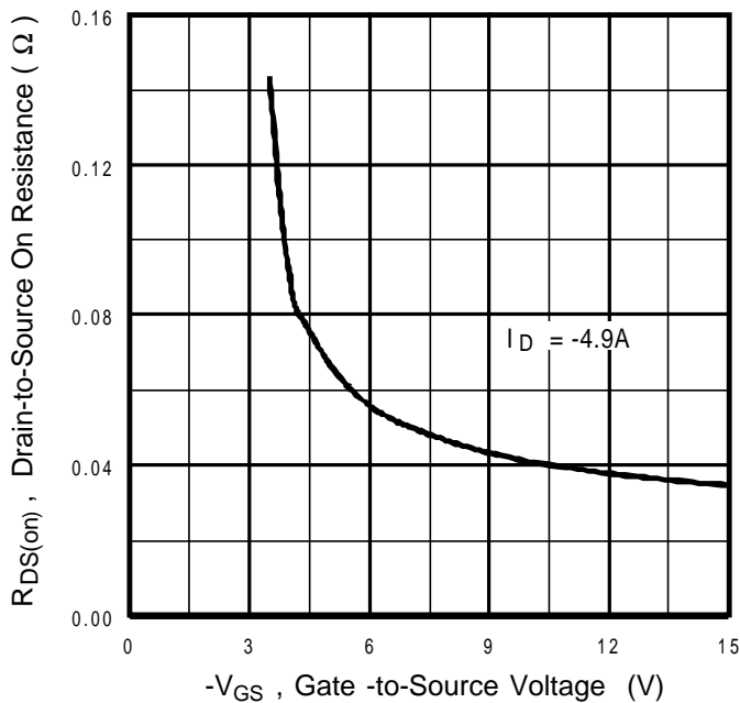
Fig 18. Typical On-Resistance Vs. Gate Voltage
