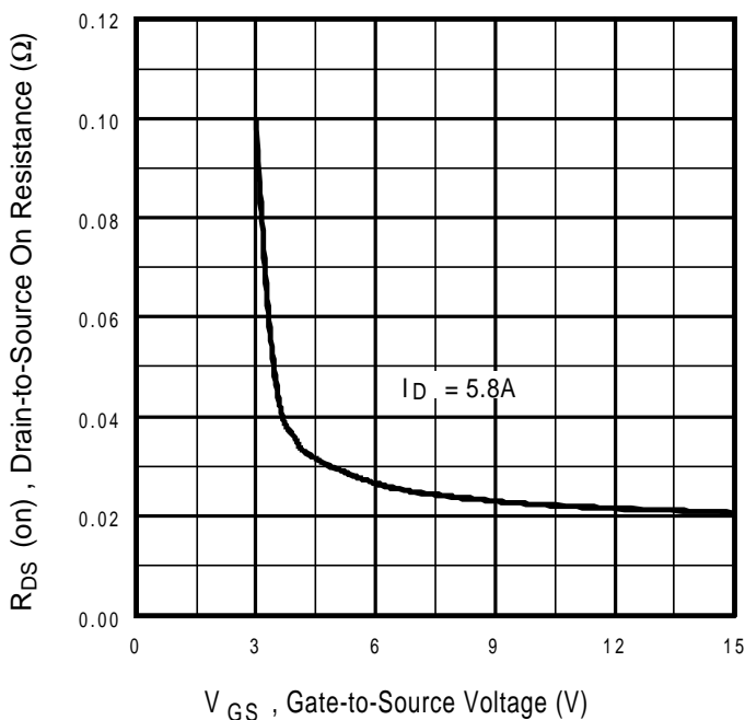
Fig 7. Typical On-Resistance Vs. Gate Voltage
