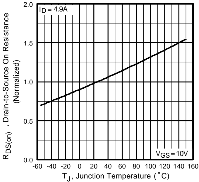
Fig 16. Normalized On-Resistance Vs. Temperature
