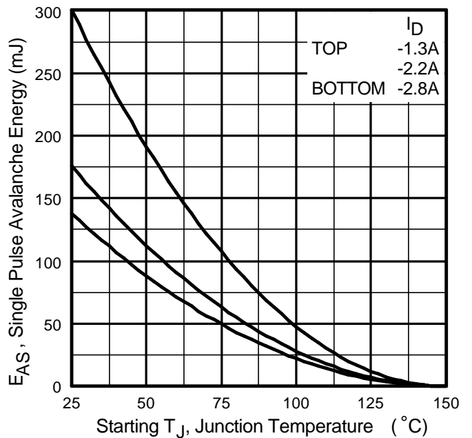
Fig 19. Maximum Avalanche Energy Vs. Drain Current
