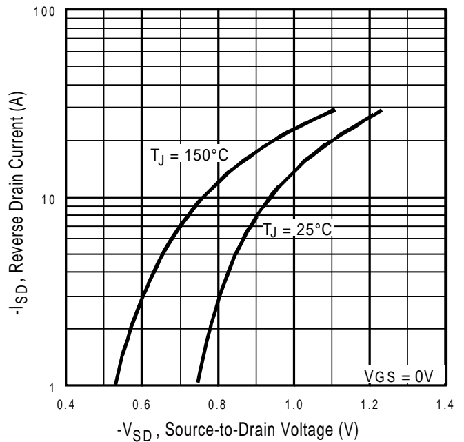
Fig 15. Typical Source-Drain Diode Forward Voltage
