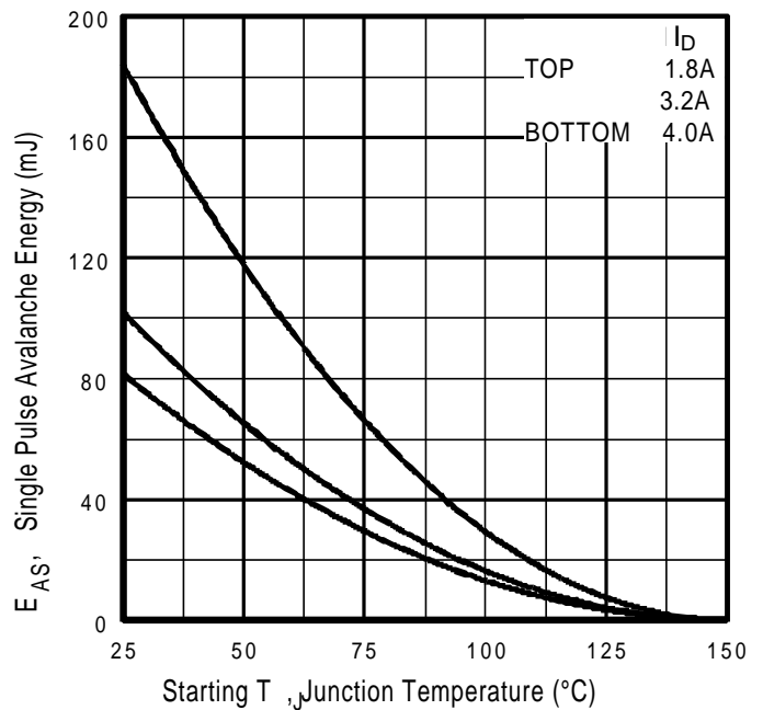
Fig 8. Maximum Avalanche Energy Vs. Drain Current
