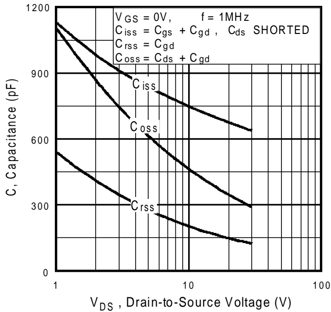
Fig 9. Typical Capacitance Vs. Drain-to-Source Voltage
