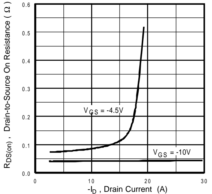
Fig 17. Typical On-Resistance Vs. Drain Current
