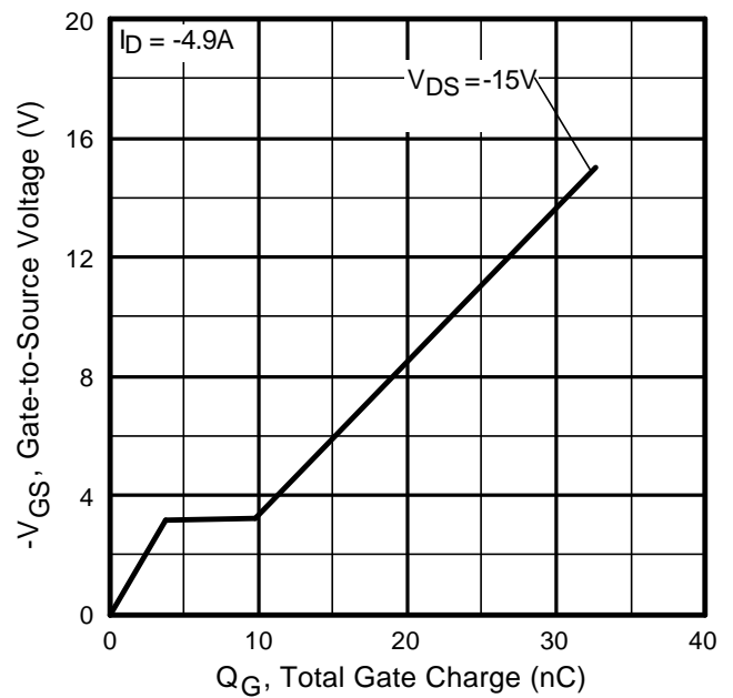
Fig 21. Typical Gate Charge Vs. Gate-to-Source Voltage
