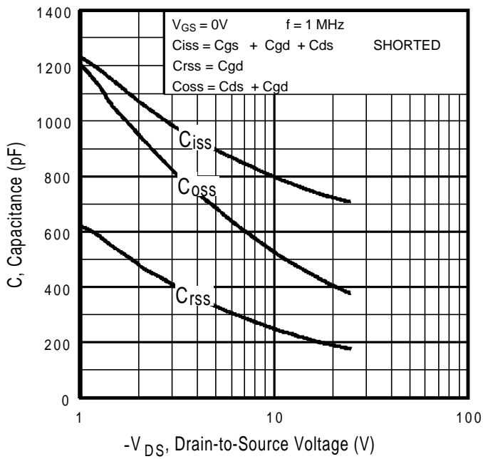
Fig 20. Typical Capacitance Vs. Drain-to-Source Voltage
