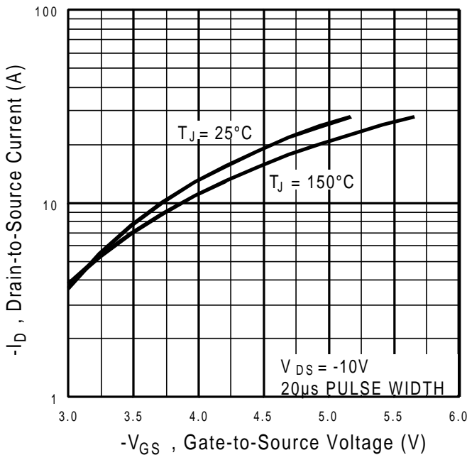
Fig 14. Typical Transfer Characteristics
