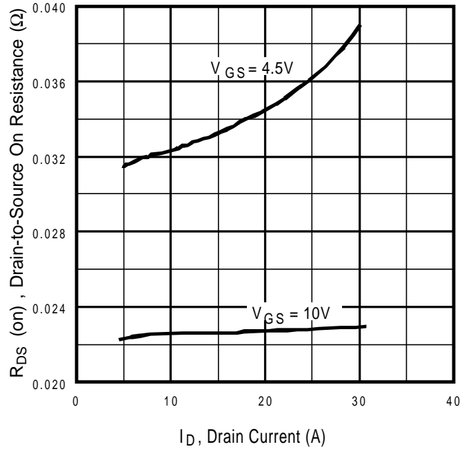
Fig 6. Typical On-Resistance Vs. Drain Current
