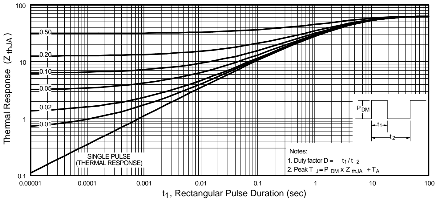
Fig 22. Maximum Effective Transient Thermal Impedance, Junction-to-Ambient
