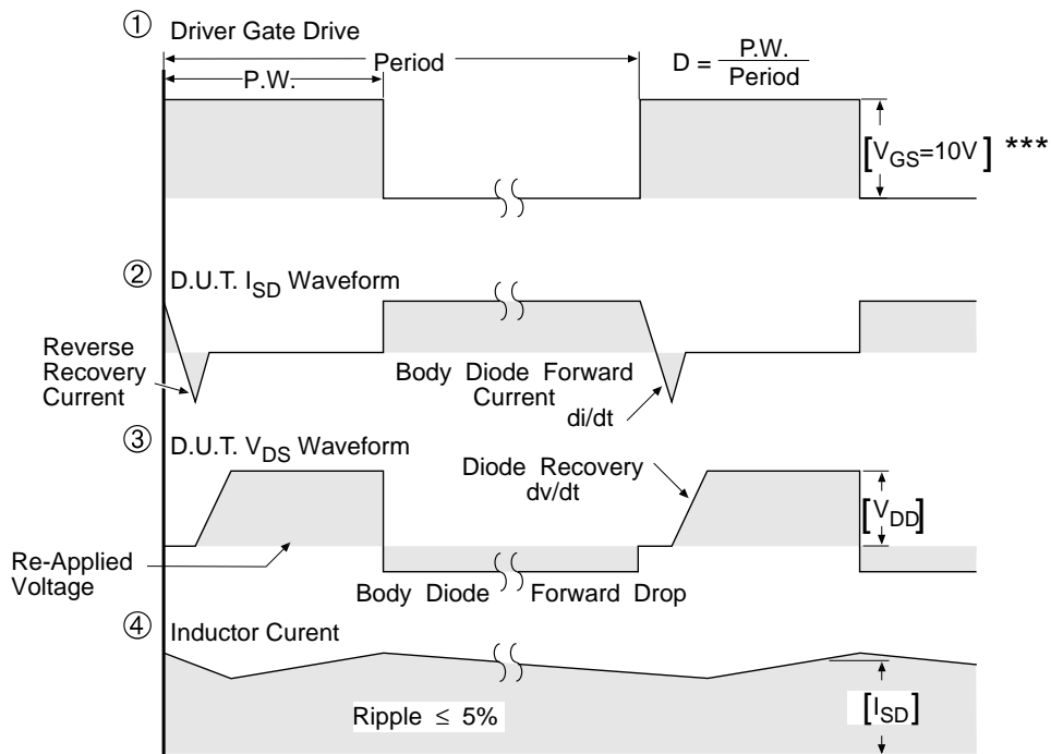
Fig 13. For P-Channel HEXFETS
