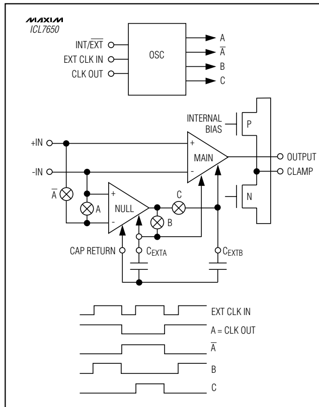
Figure 2. Block Diagram
