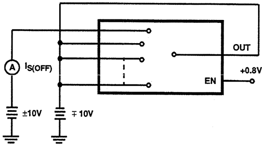
FIGURE 2C. I_{S(\text{OFF})} TEST CIRCUIT (NOTE 1)
