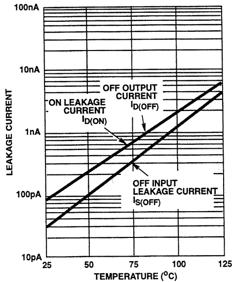
FIGURE 2A. LEAKAGE CURRENT vs TEMPERATURE
