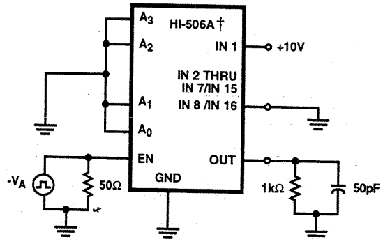
† Similar connection for HI-507A/HI-508A/HI-509A
