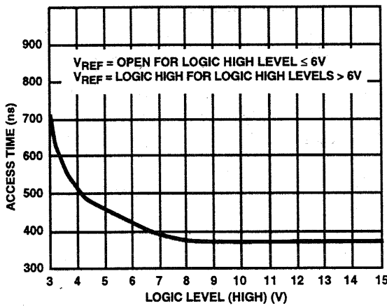
FIGURE 6A. ACCESS TIME vs LOGIC LEVEL (HIGH)
