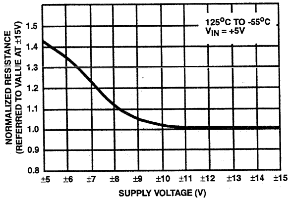
FIGURE 1C. NORMALIZED ON RESISTANCE vs SUPPLY VOLTAGE
