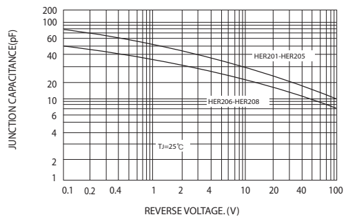
FIG.6-TYPICAL JUNCTION CAPACITANCE
