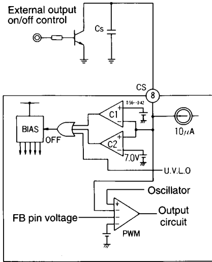
Fig. 13 External output on/off control circuit
