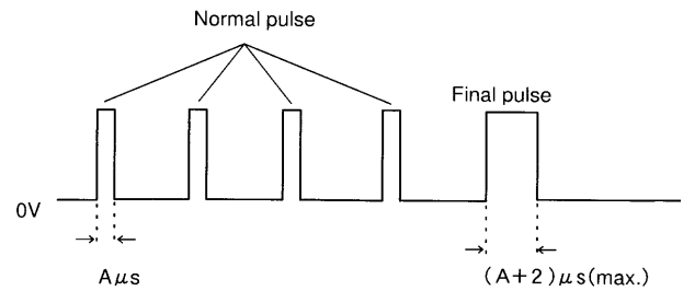
Fig. 29 OUT terminal voltage waveform
