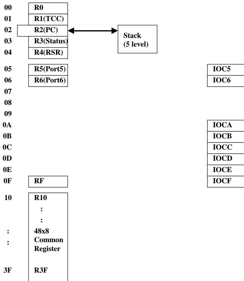
Fig. 4 Data Memory Configuration
