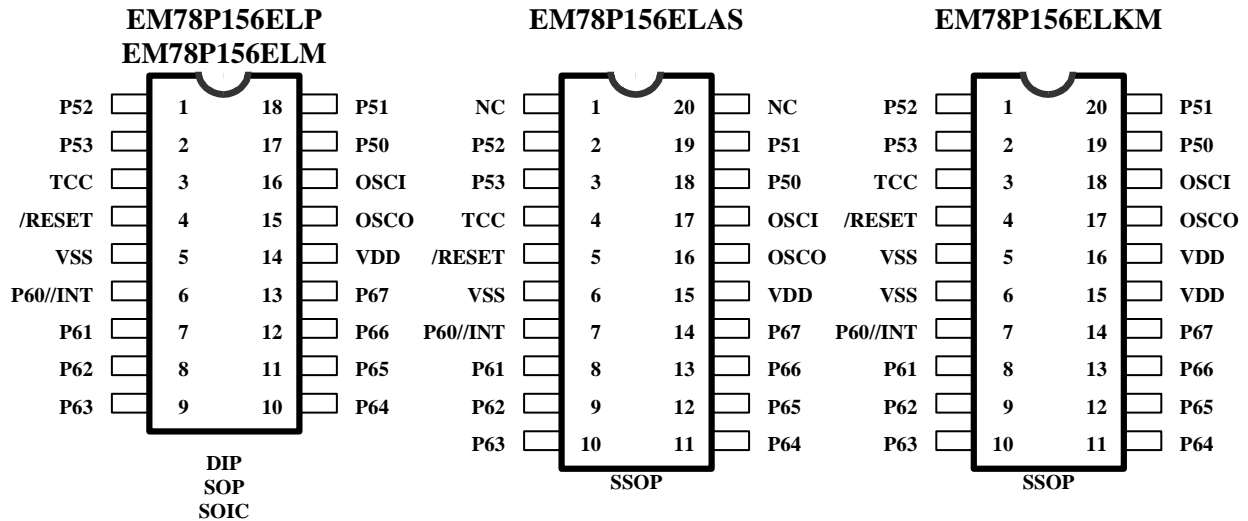
Fig. 1 Pin Assignment
