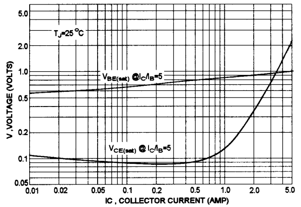
"ON" VOLTAGES
