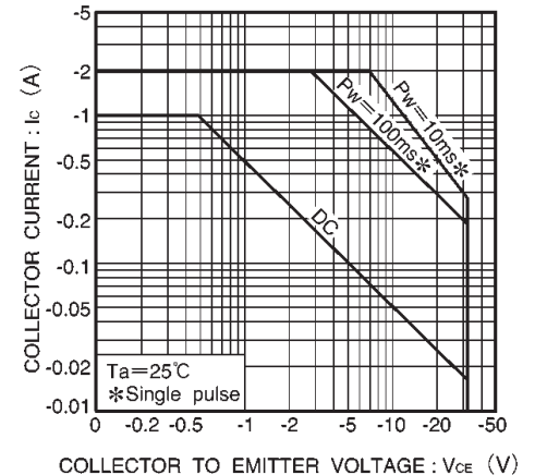
Fig.9 Safe operation area (2SB1132)
