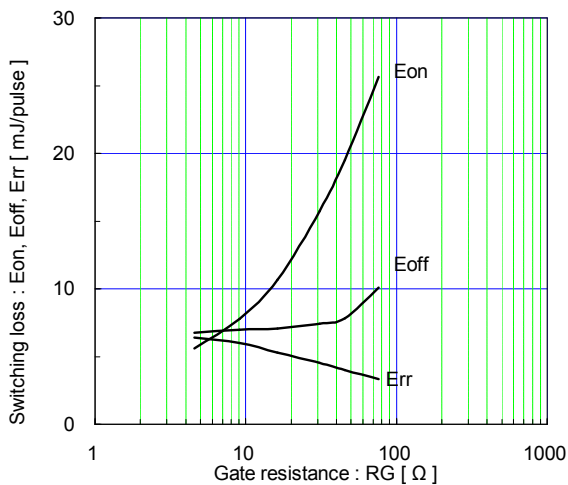
Switching loss vs. Gate resistance (typ.) V_{CC}=600V, I_C=75A, V_{GE}=\pm 15V, T_J=25^\circ C
