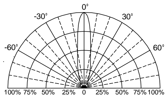
Fig.6 Directive Radiation
