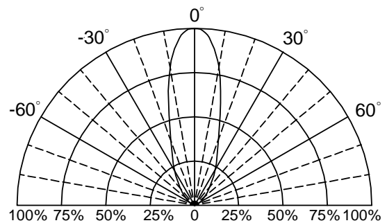
Fig.6 Directivity Radiation
