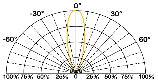
Fig.6 Directivity Radiation
