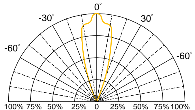
Fig.6 Directivity Radiation
