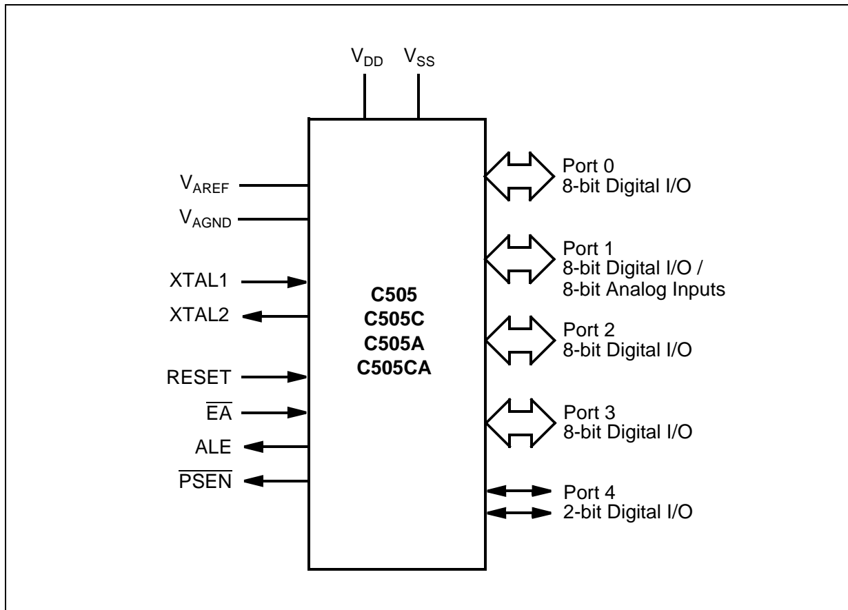
Figure 2 Logic Symbol
