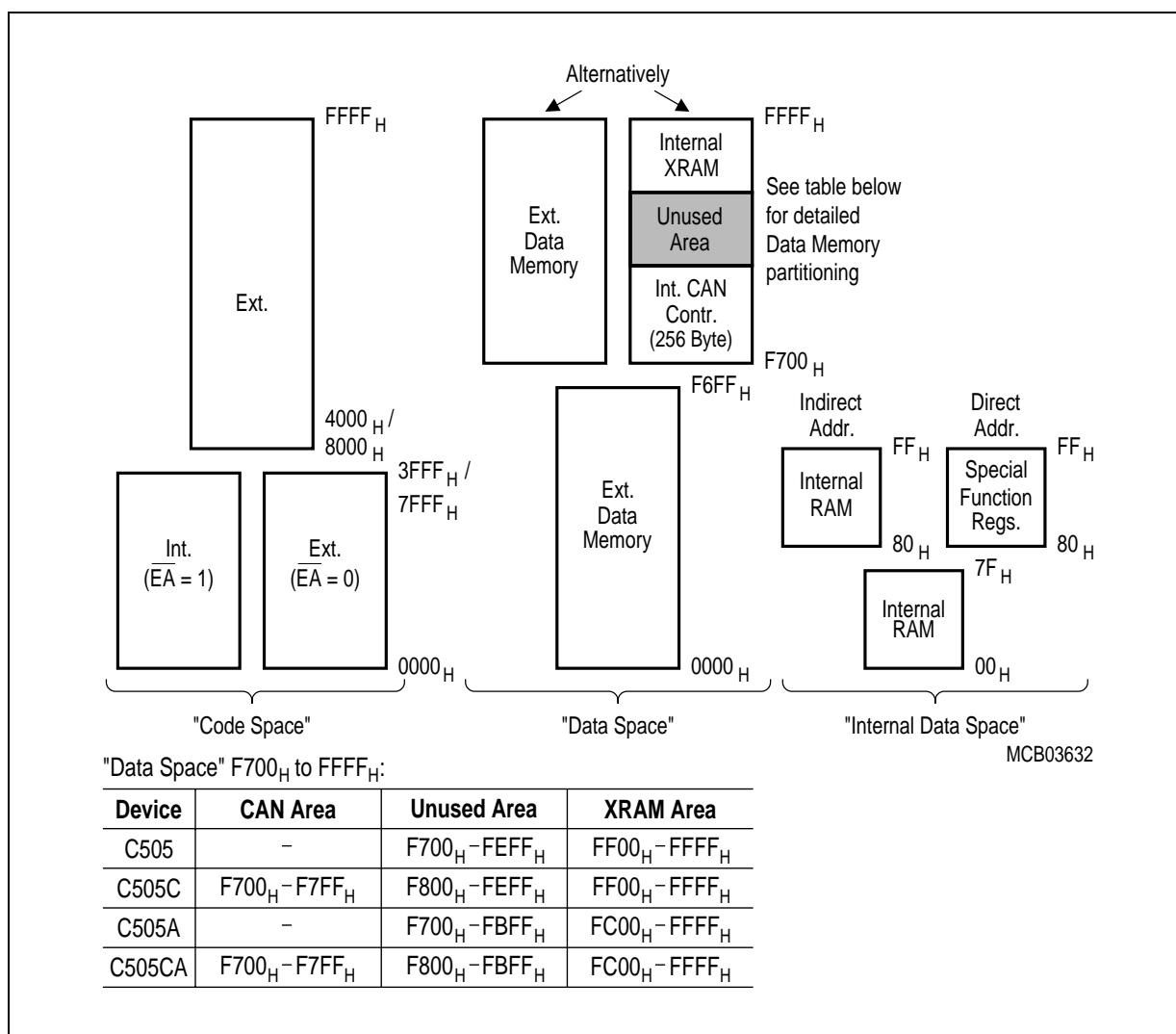
Figure 5 C505 Memory Map
