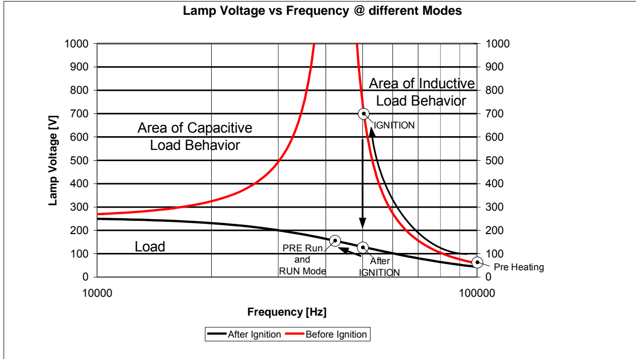
Figure 21 Capacitive and Inductive Operation
