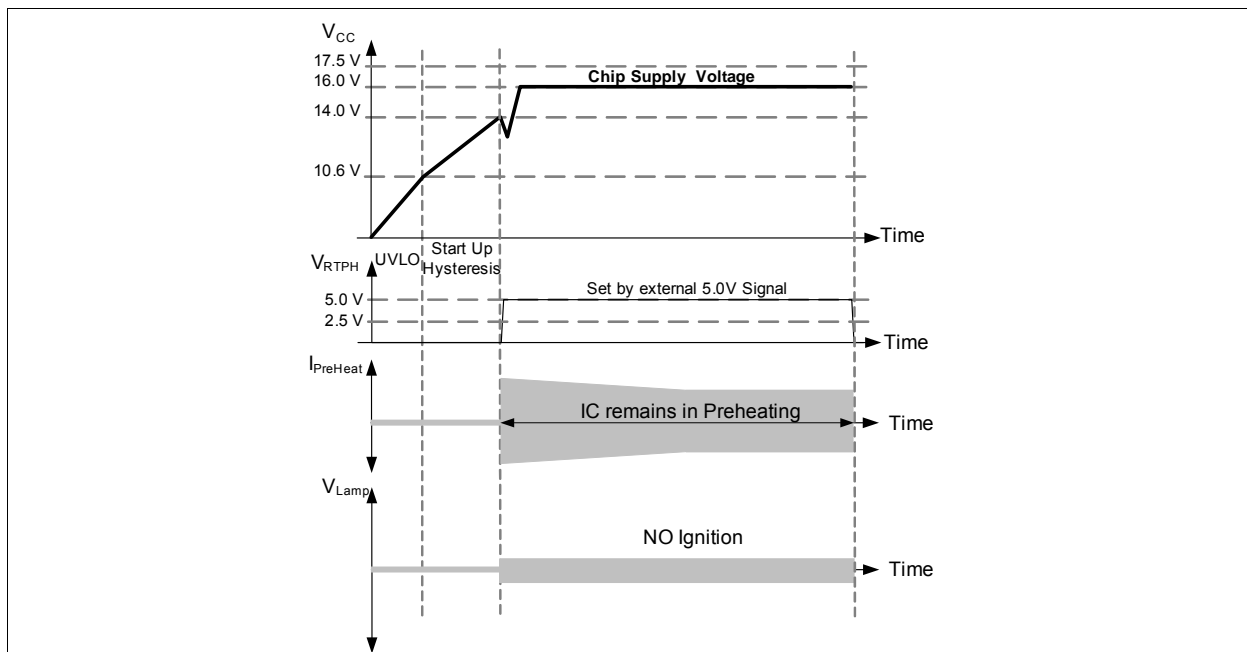
Figure 30 Start-Up WITHOUT Preheating
