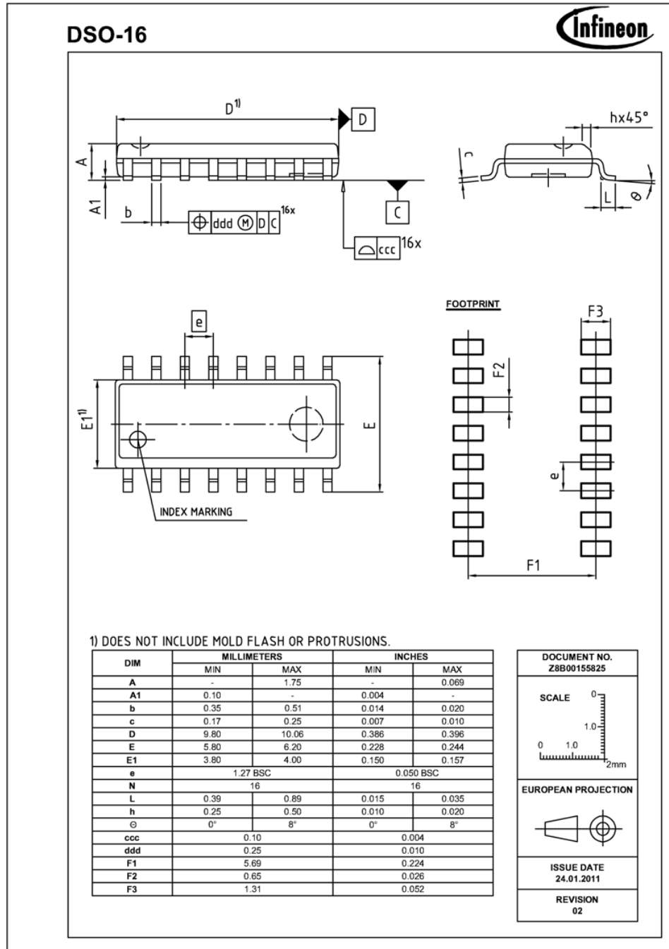
Figure 40 Package Outline with Creep Distance
