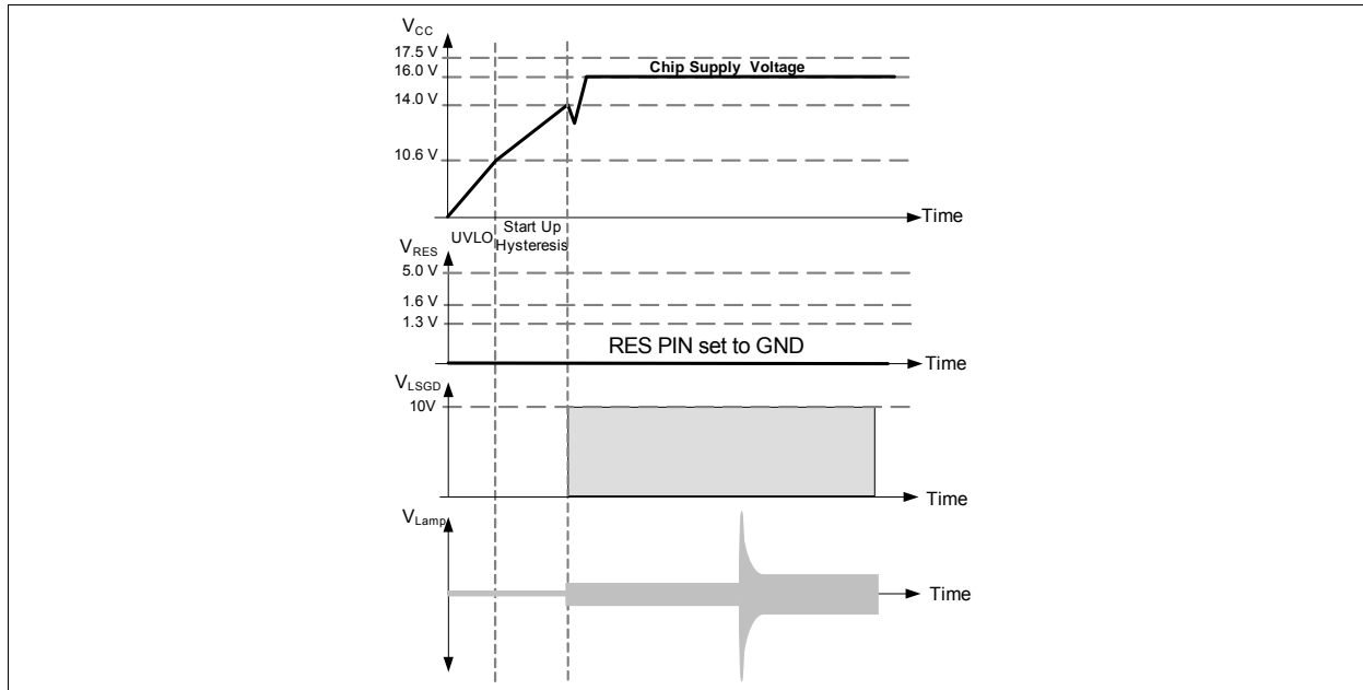
Figure 31 Deactivation via RES PIN
