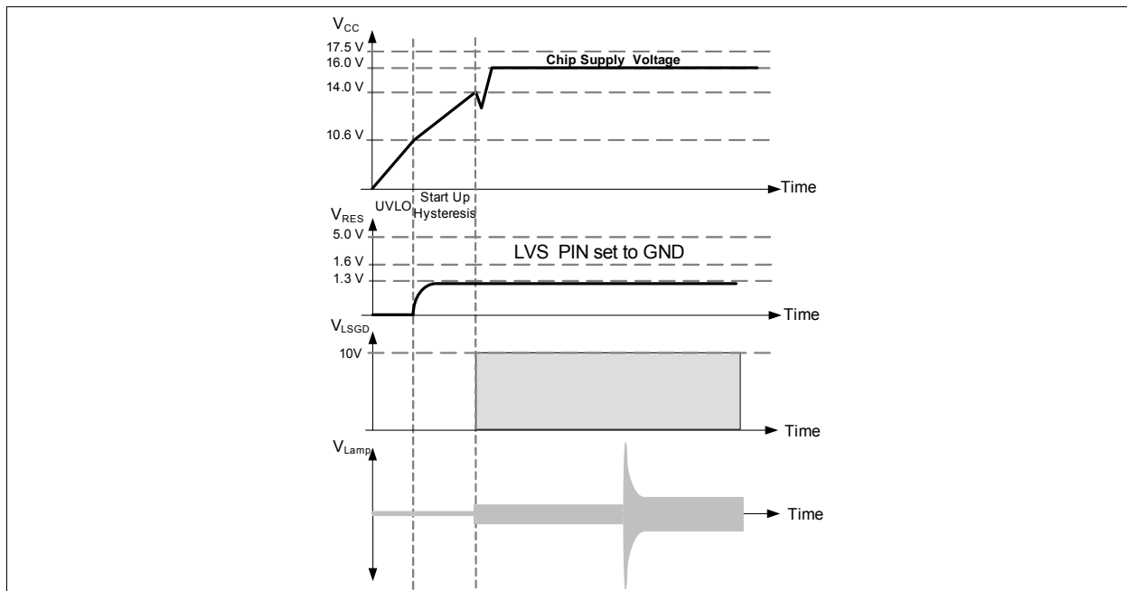
Figure 32 Deactivation via LVS PIN
