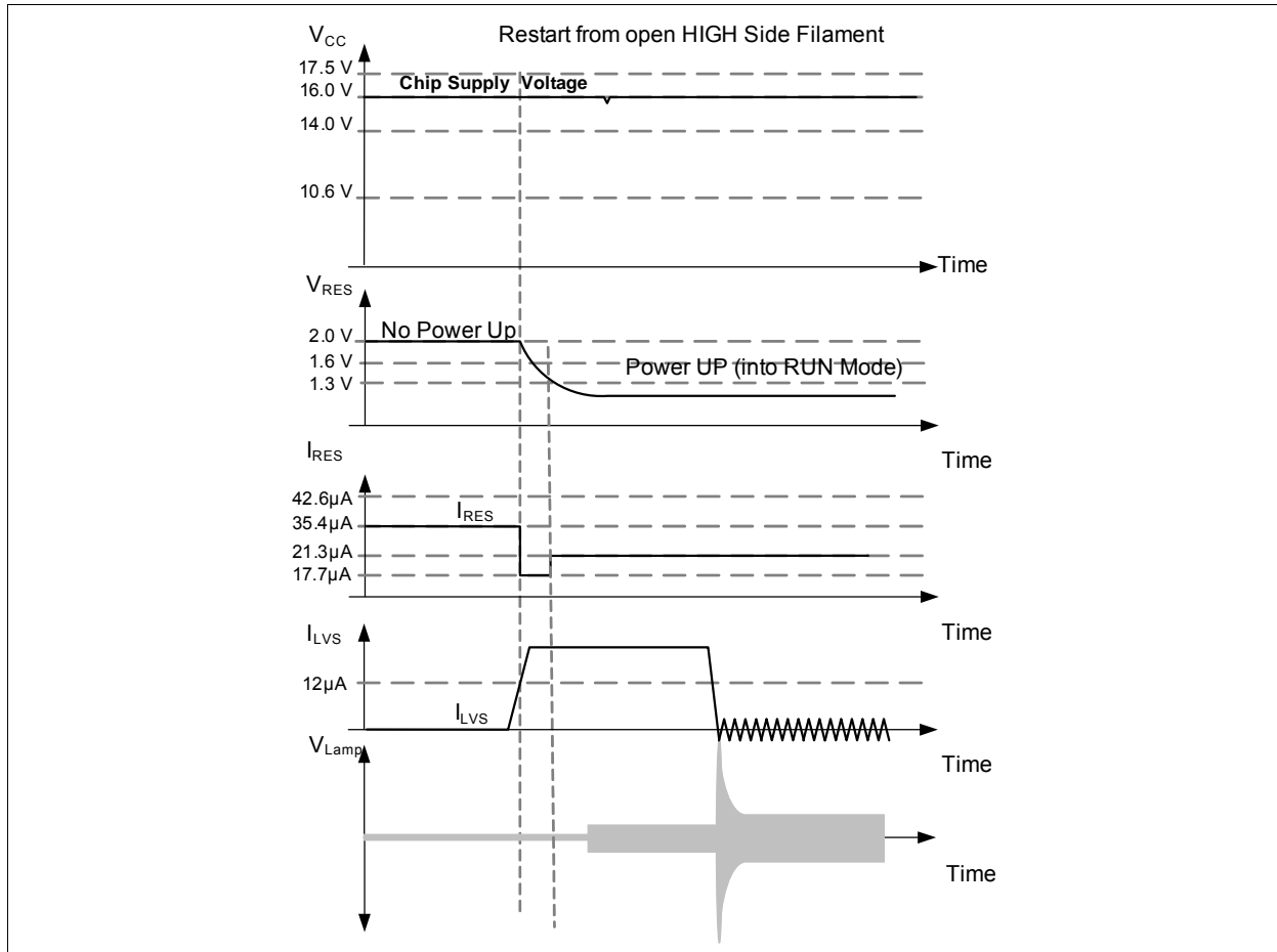
Figure 13 Restart from Open High Side Filament
