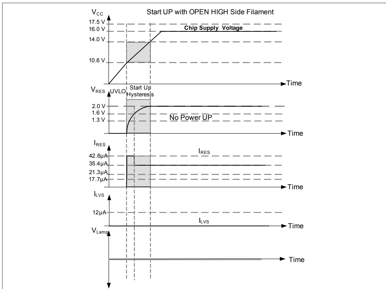
Figure 12 Start-Up with Open High Side Filament
