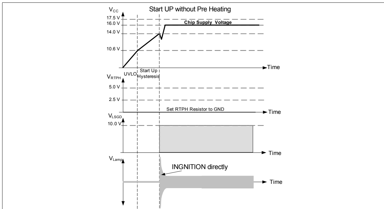
Figure 28 Start-Up WITHOUT Preheating
