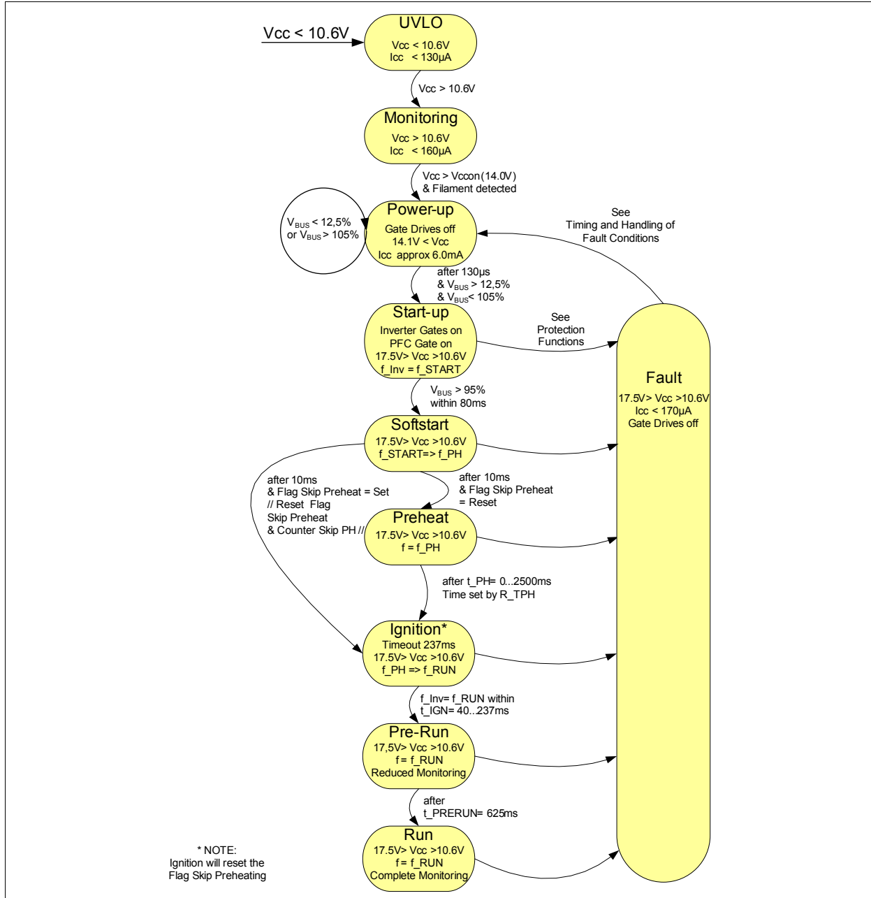
Figure 35 Operating Flow during Start-Up Procedure
