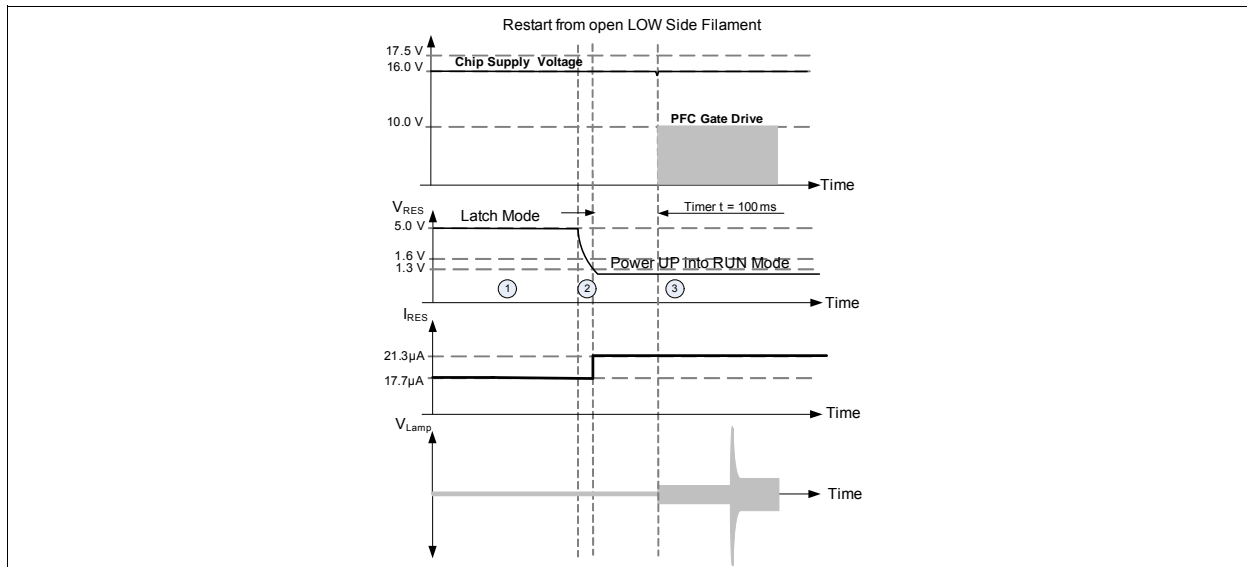
Figure 9 Restart from Open Low Side Filament
