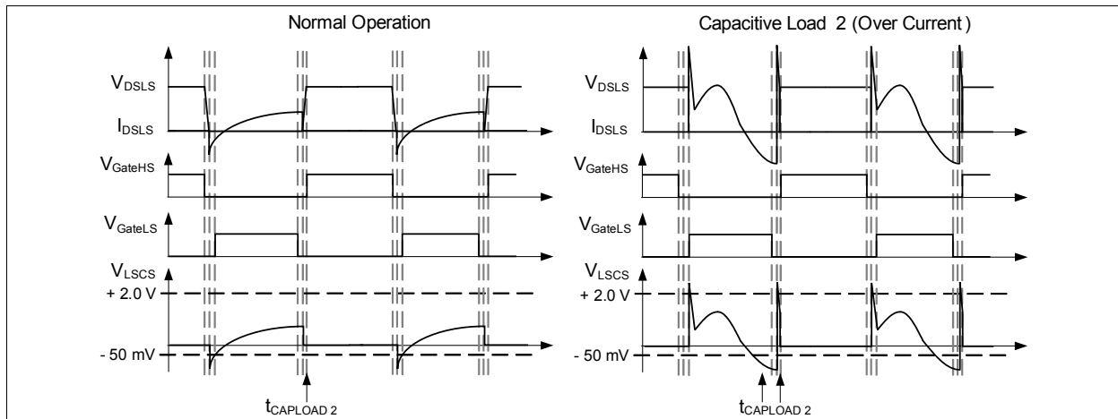
Figure 23 Capacitive Mode 2 – Operation with Overcurrent
