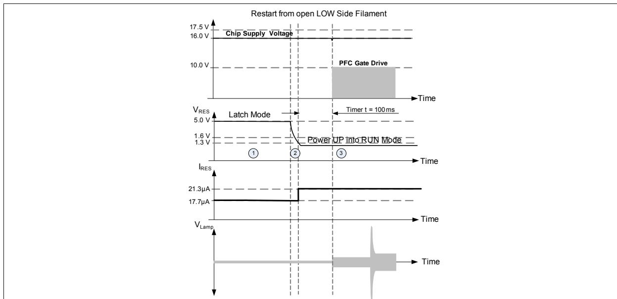
Figure 11 Restart from Open LS Filament
