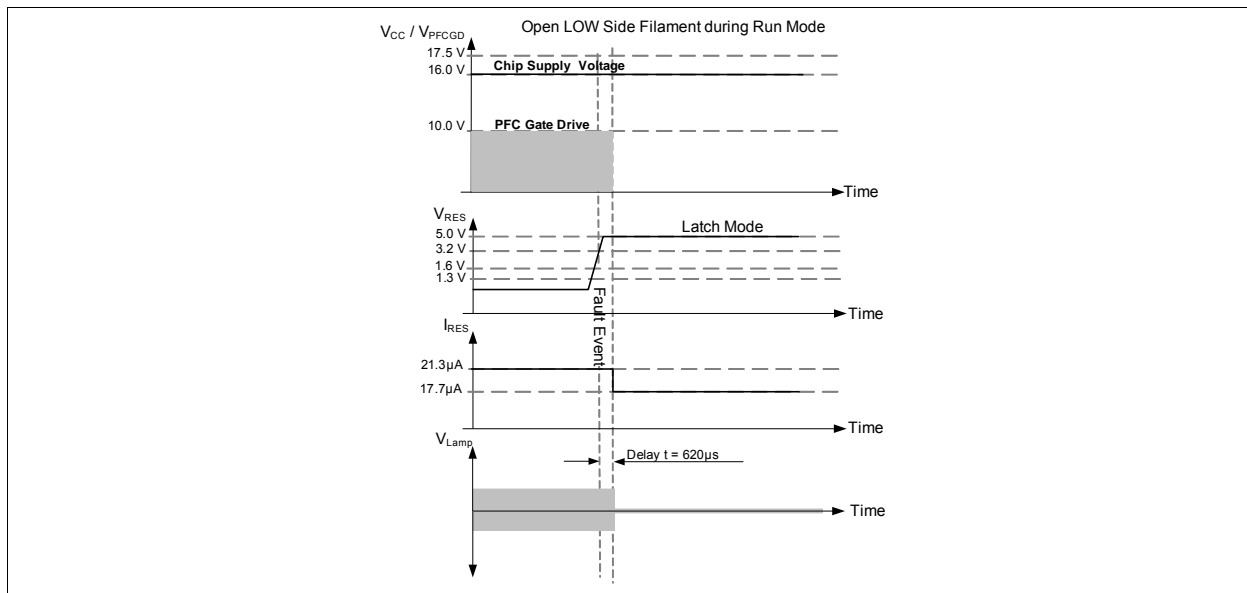
Figure 10 Open Low Side Filament Run Mode
