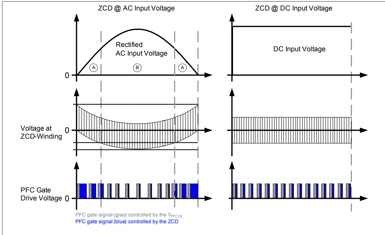
Figure 17 THD Optimization using adjustable Pulse Width Extension
