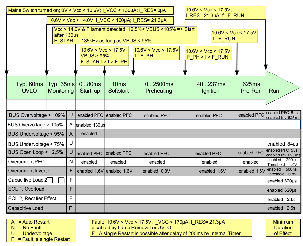
Figure 34 Monitoring Features during Different Operating Modes
