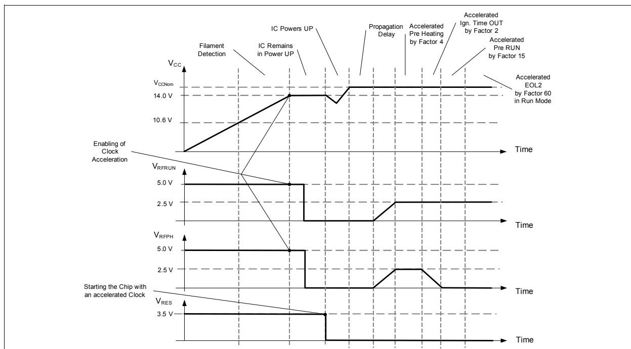
Figure 33 Clock Acceleration (Built in Customer Test Mode)
