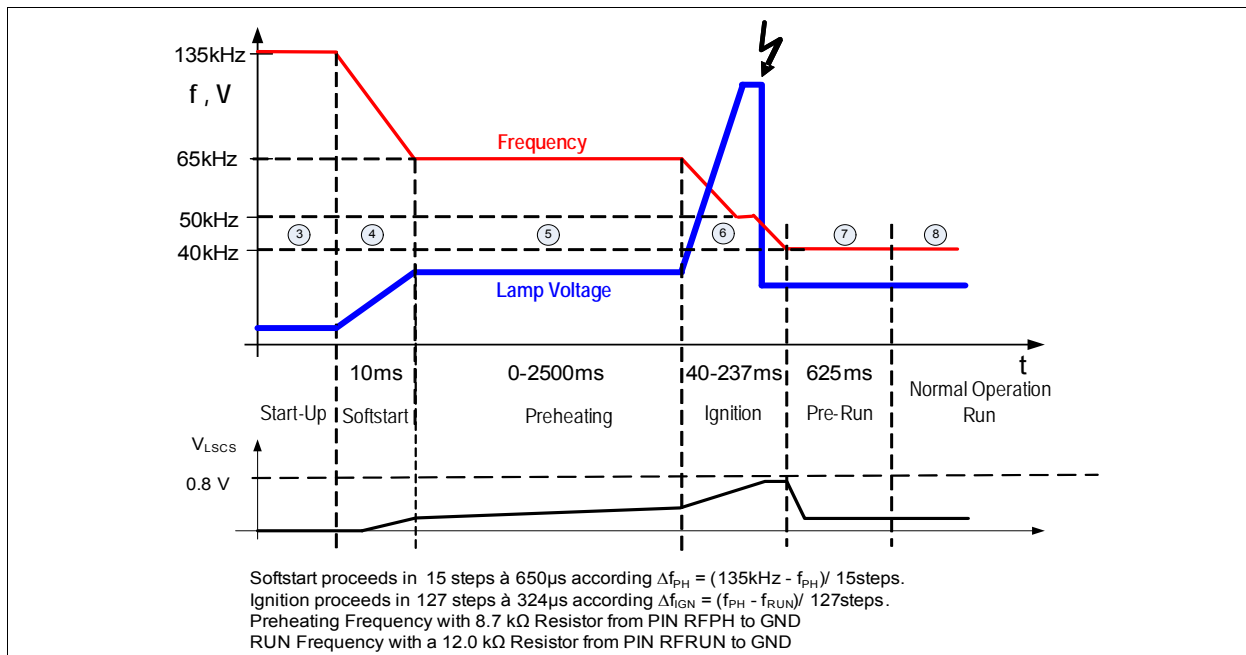
Figure 6 Typical Variation of Operating Frequency during Startup
