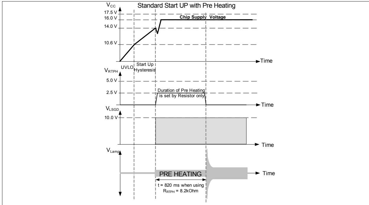
Figure 27 Start-Up WITH Preheating
