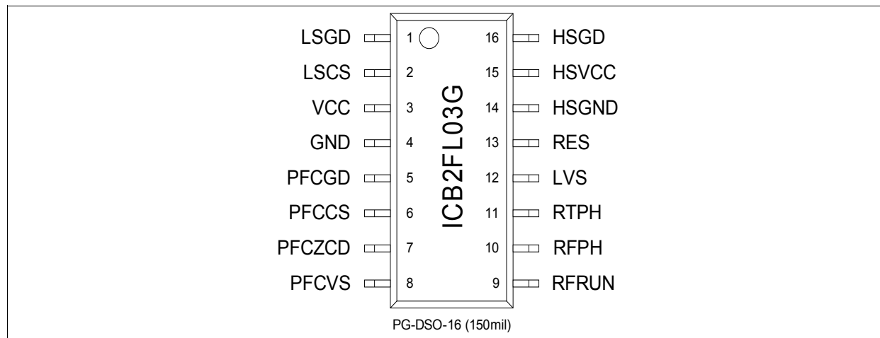
Figure 2 PG-DSO-16-20 Package (top view)
