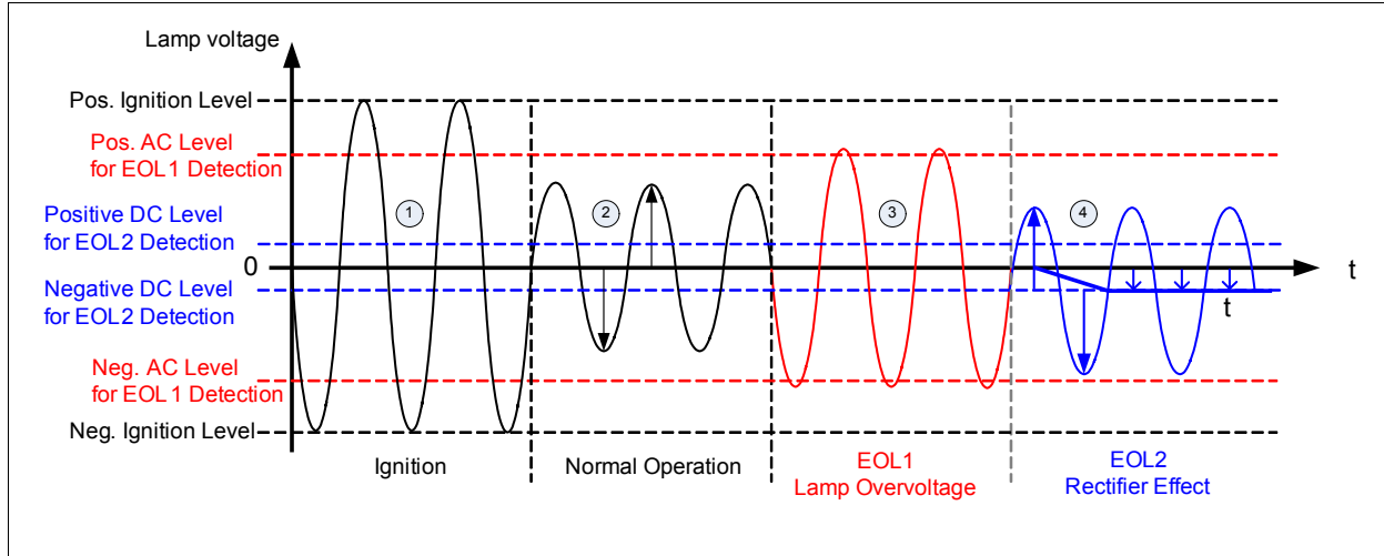
Figure 18 End of Life and Rectifier Effect
