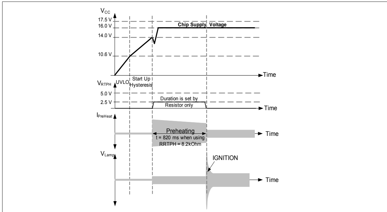
Figure 29 Start-Up WITH Preheating
