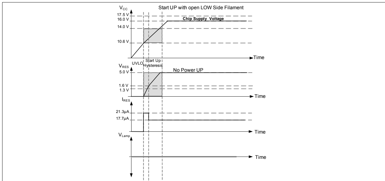
Figure 8 Start-Up with Open Low Side Filament
