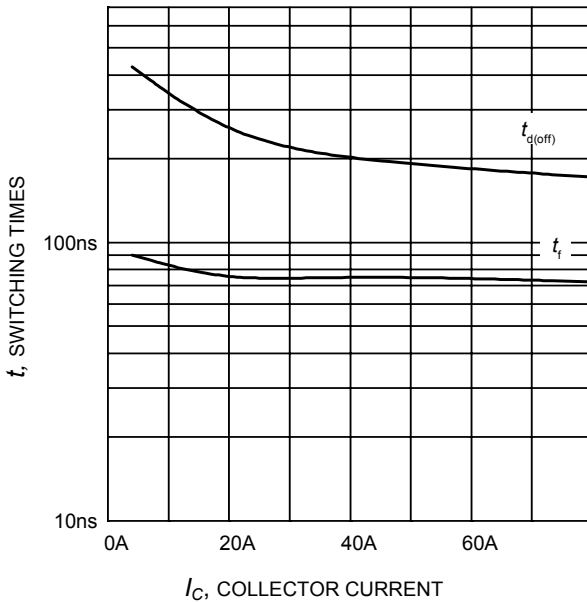
Figure 9. Typical switching times as a function of collector current (inductive load, T_J=175^\circ\text{C} , V_{CE} = 400\text{V} , V_{GE} = 0/15\text{V} , R_G = 5.6\Omega , Dynamic test circuit in Figure E)
