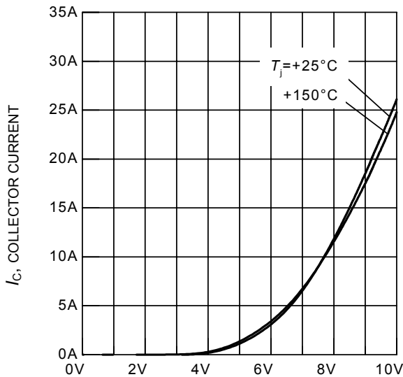
V_{GE} , GATE-EMITTER VOLTAGE Figure 7. Typical transfer characteristics ( V_{CE} = 10\text{V} )
