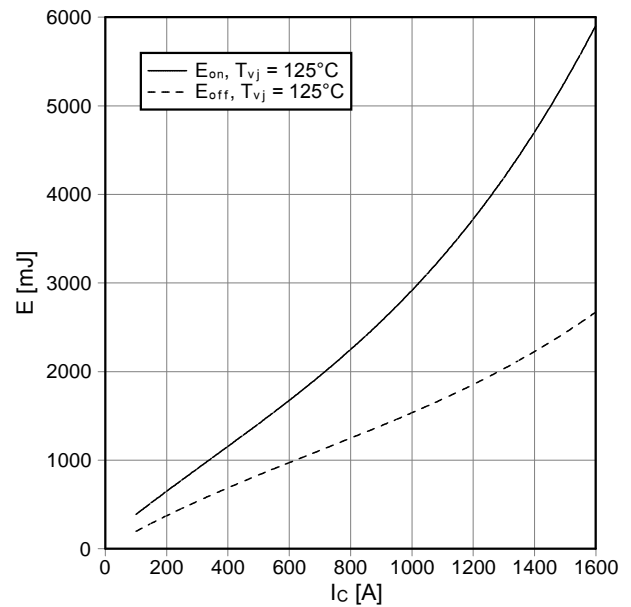
Schaltverluste IGBT-Wechselr. (typisch) switching losses IGBT-inverter (typical) E_{on} = f(I_c) , E_{off} = f(I_c) V_{GE} = \pm 15\text{ V} , R_{Gon} = 3\ \Omega , R_{Goff} = 6,8\ \Omega , V_{CE} = 1800\text{ V} , C_{GE} = 220\text{ nF}
