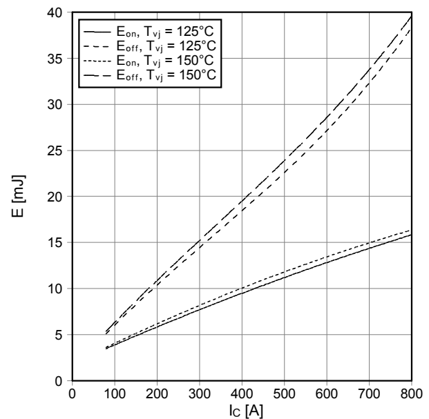
Schaltverluste IGBT-Wechselr. (typisch) switching losses IGBT-inverter (typical) E_{on} = f(I_c) , E_{off} = f(I_c) V_{GE} = \pm 15\text{ V} , R_{Gon} = 1.8\ \Omega , R_{Goff} = 0.75\ \Omega , V_{CE} = 300\text{ V}
