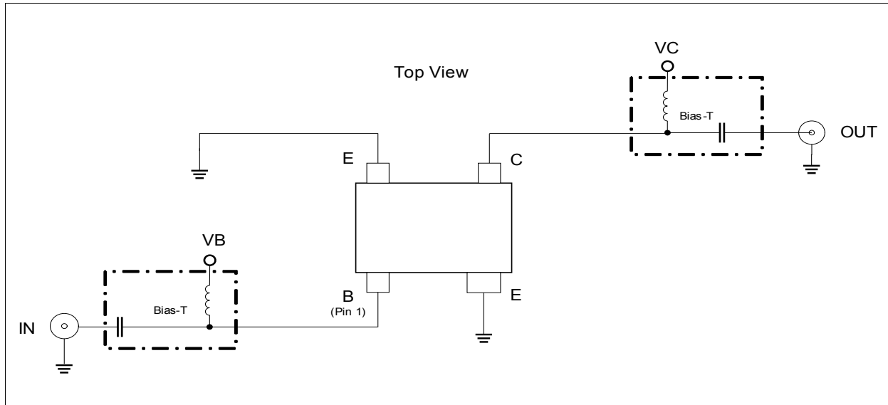
Figure 2 BFP740ESD Testing Circuit
