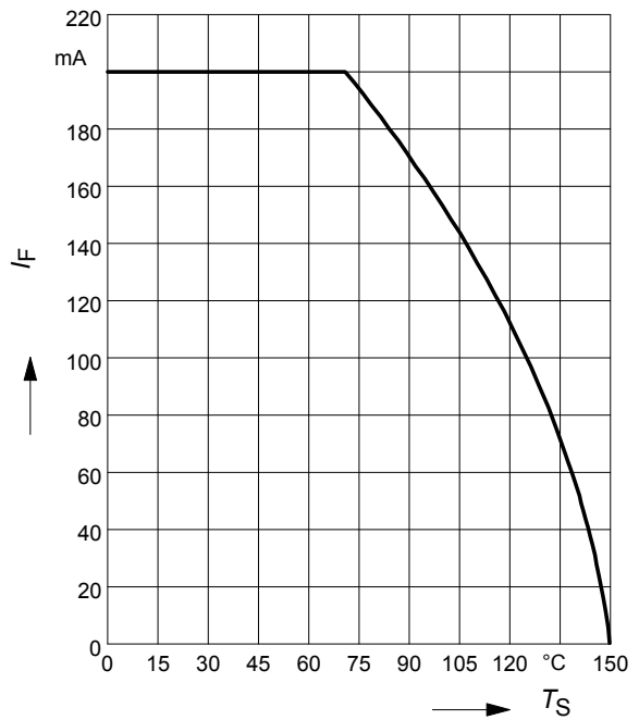
BAT54-05W
