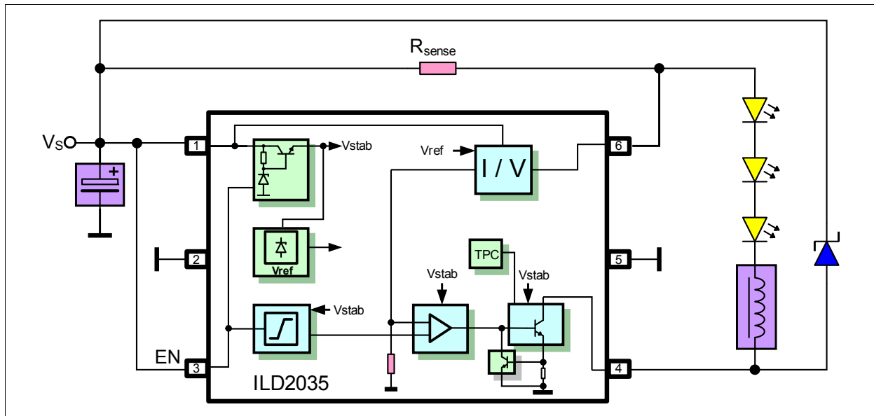
Figure 4 Application Circuit
