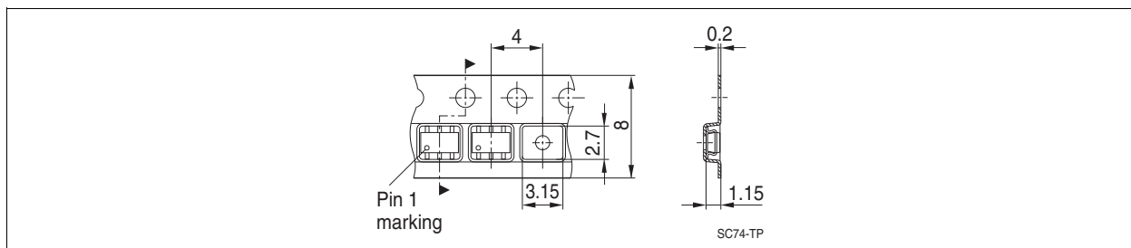
Figure 8 Tape Loading
