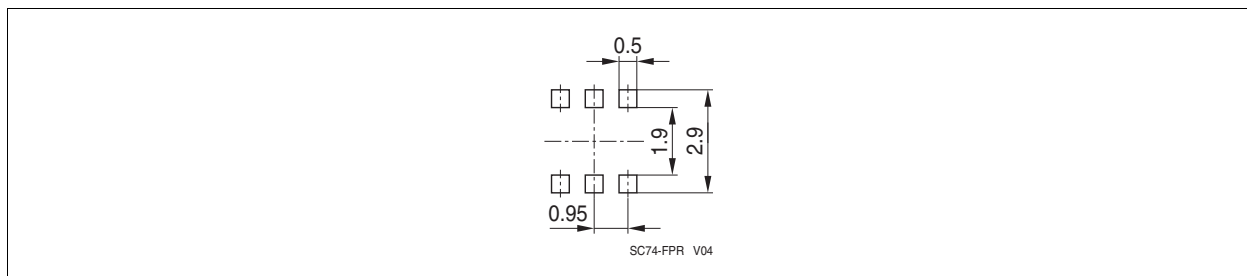
Figure 7 Recommended PCB Footprint for Reflow Soldering
