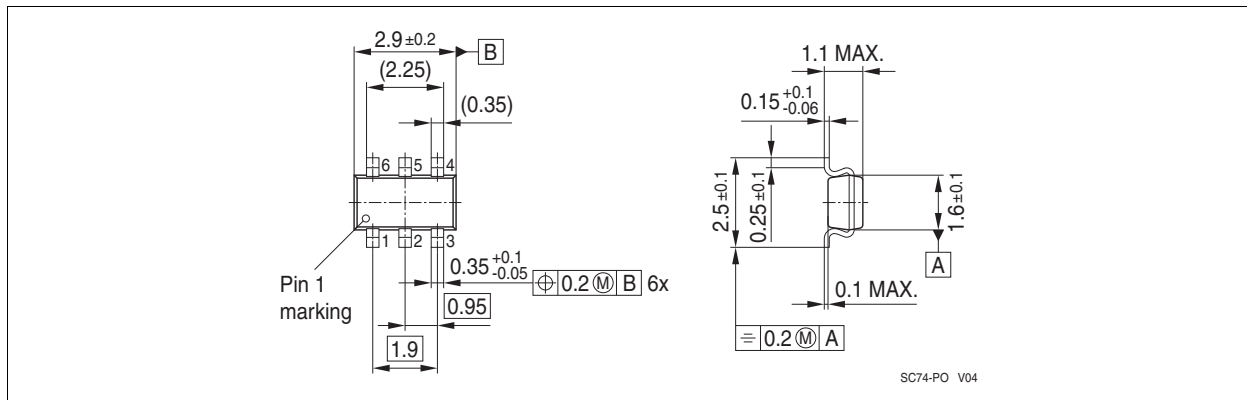
Figure 6 Package Outline SC74
