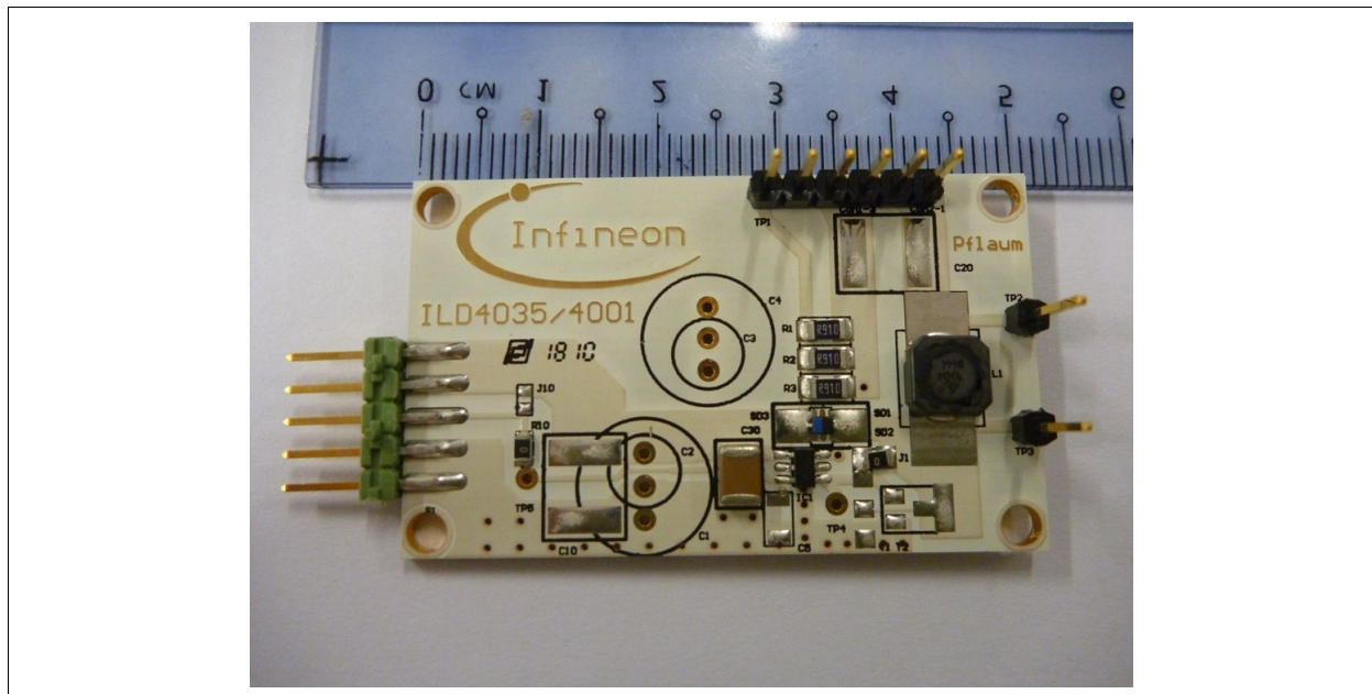
Figure 5 ILD2035 on Evaluation Board
