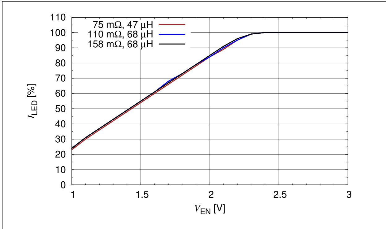
Figure 4 Analog Voltage Dimming (Relative) vs. R_{sense}
