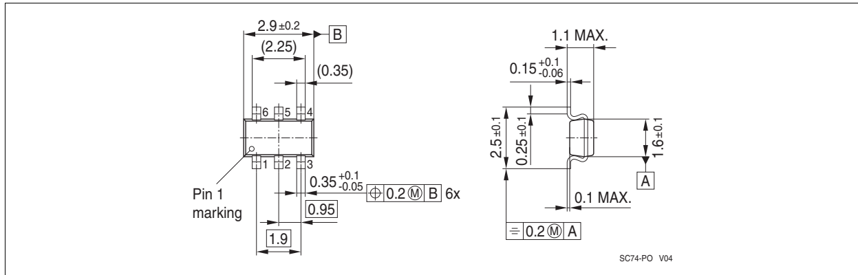
Figure 9 Package Outline SC74
