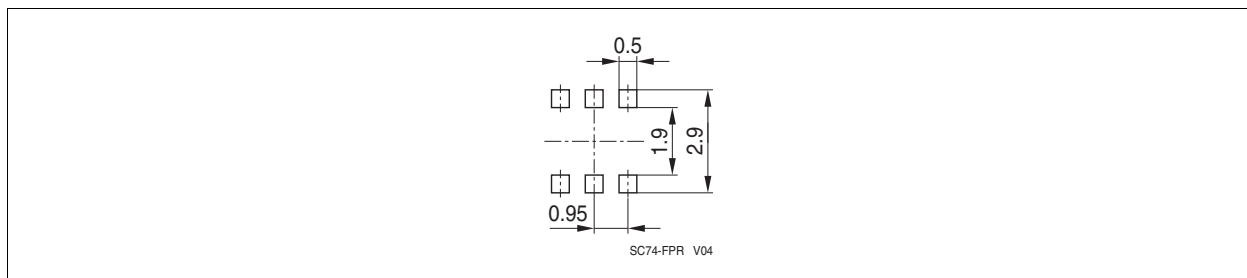
Figure 10 Recommended PCB Footprint for Reflow Soldering
