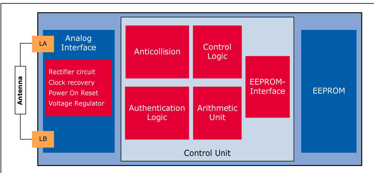
Figure 6 Block Diagram
