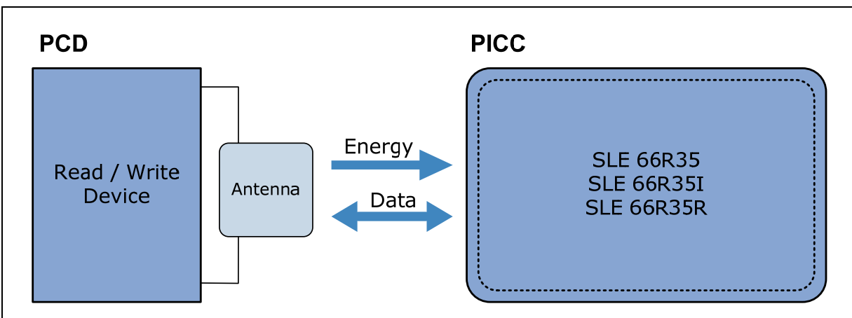
Figure 5 System Overview
