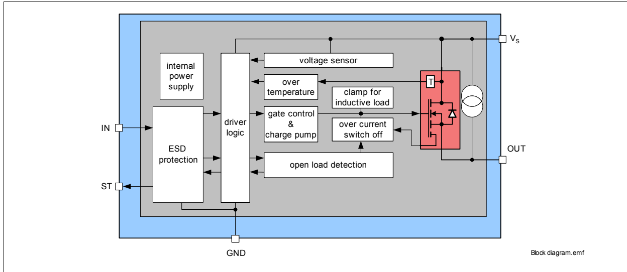
Figure 1 Block diagram for the BTS4300SGA
