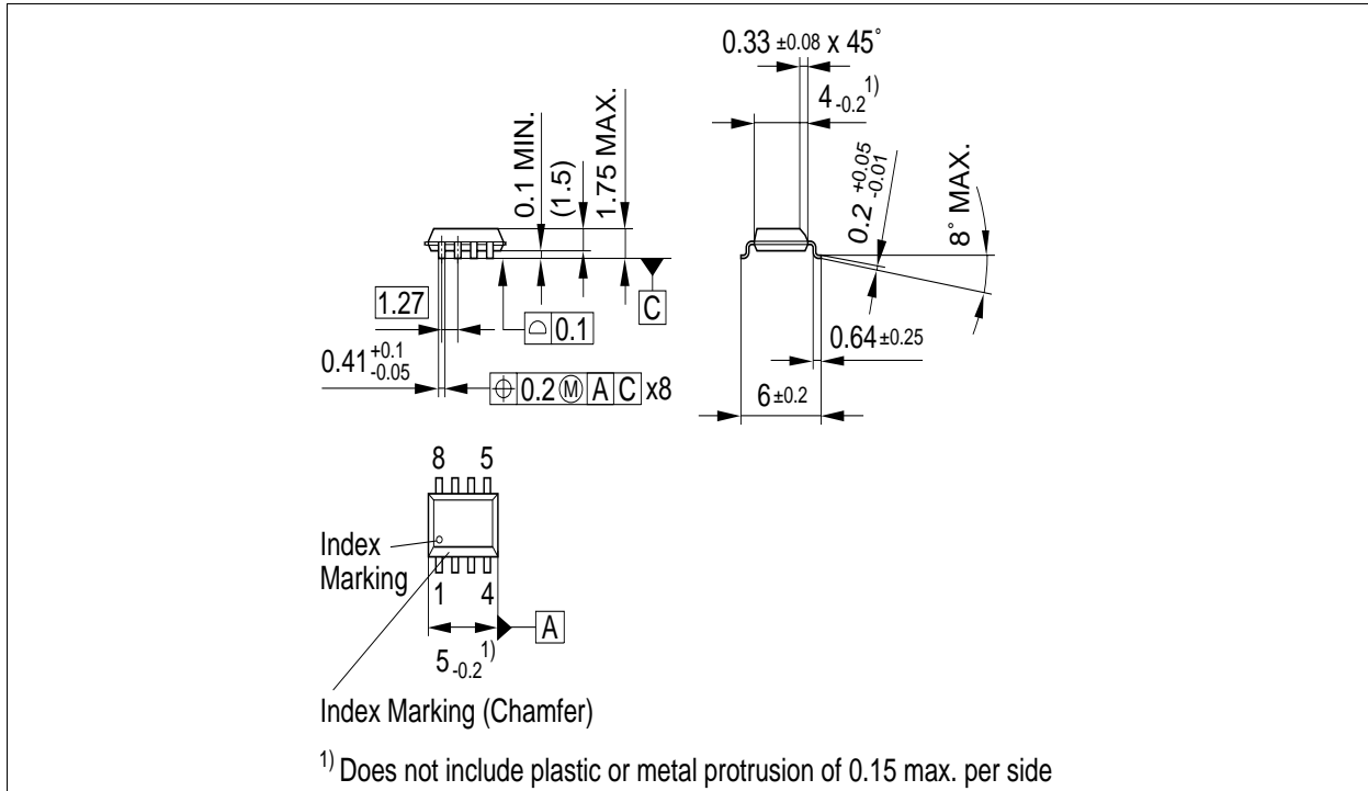
Figure 17 PG-DSO-8-24 (Plastic Dual Small Outline Package)
