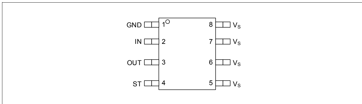
Figure 2 Pin Configuration
