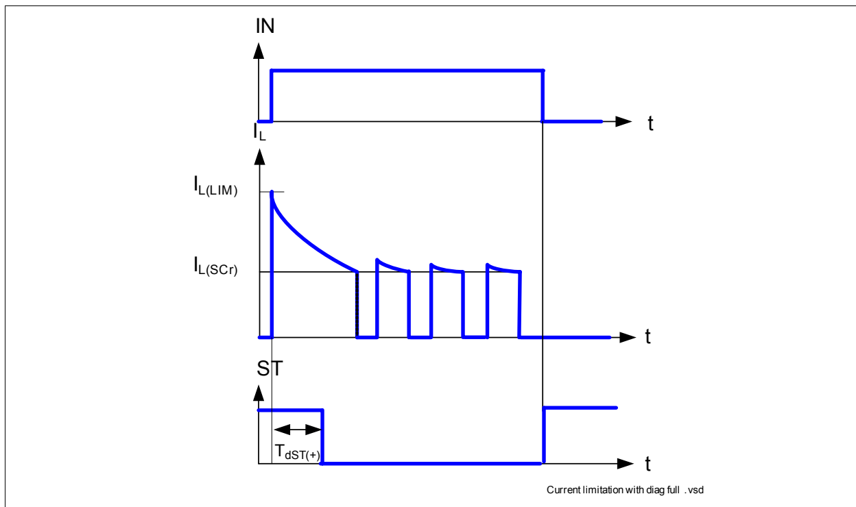
Figure 10 Current limitation function of the time
