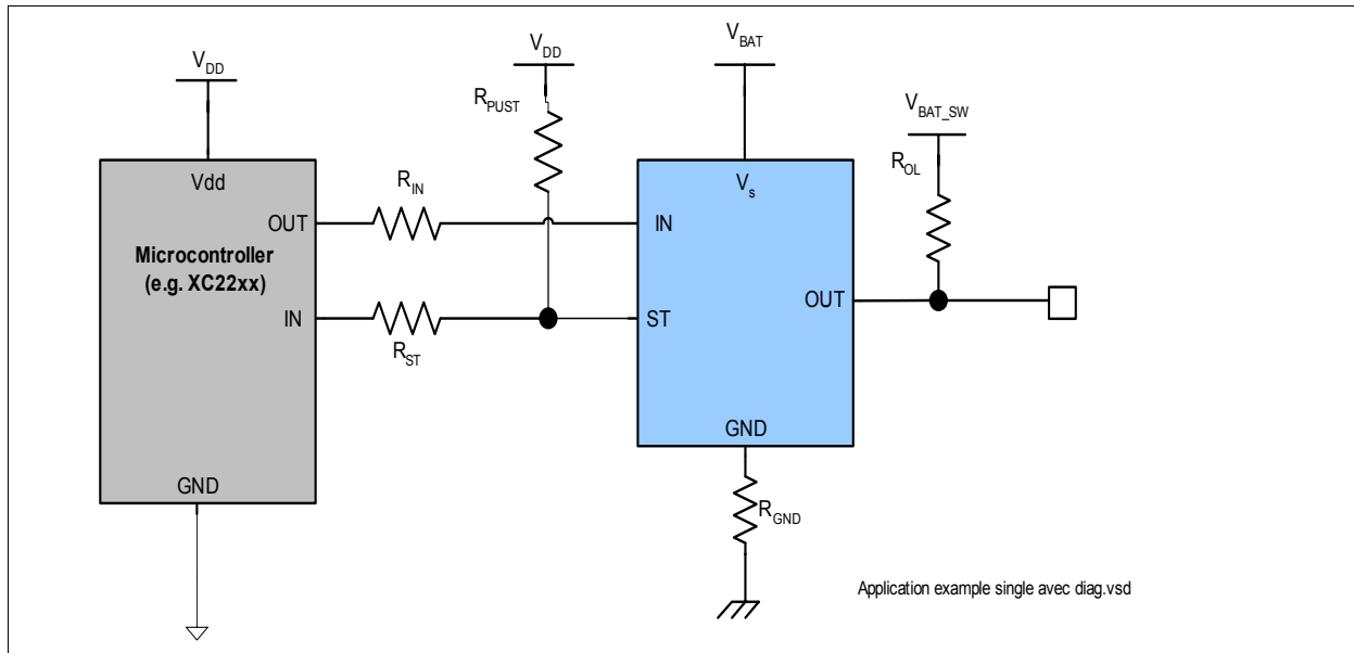
Figure 16 Application diagram with BTS4300SGA
