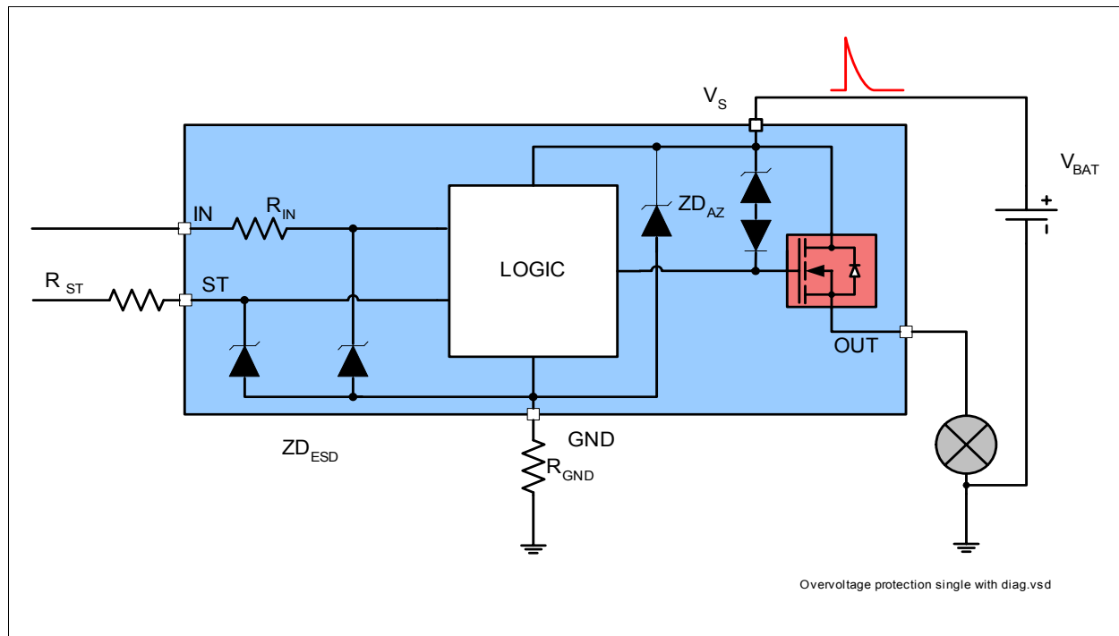
Figure 8 Over voltage protection with external components
