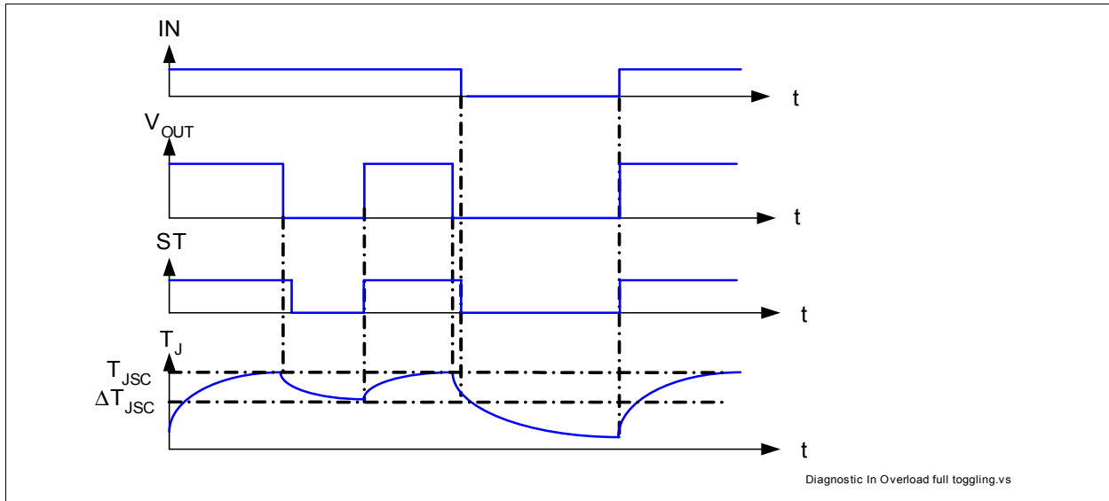
Figure 14 Sense signal in overtemperature condition
