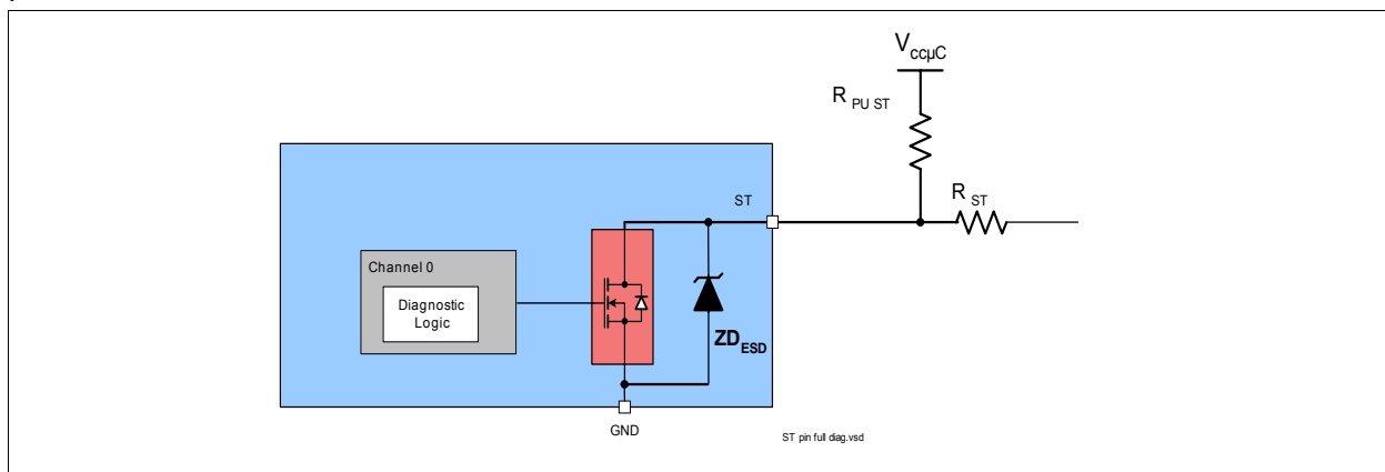
Figure 11 Status output circuitry
