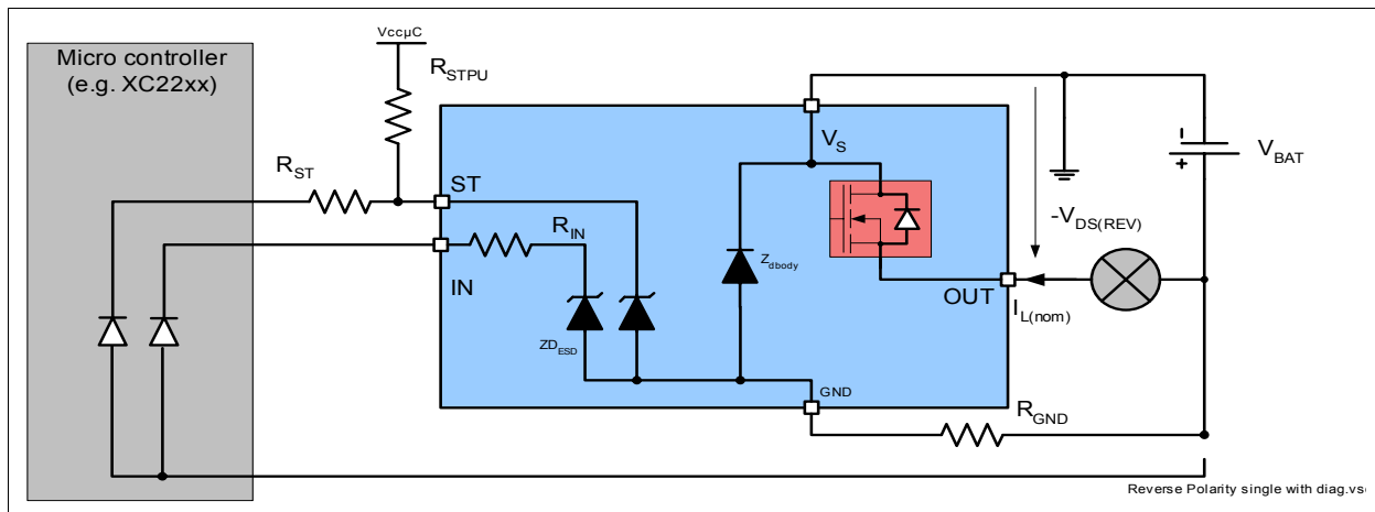
Figure 9 Reverse polarity protection with external components
