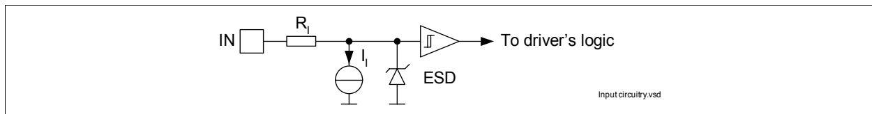
Figure 15 Input pin circuitry
