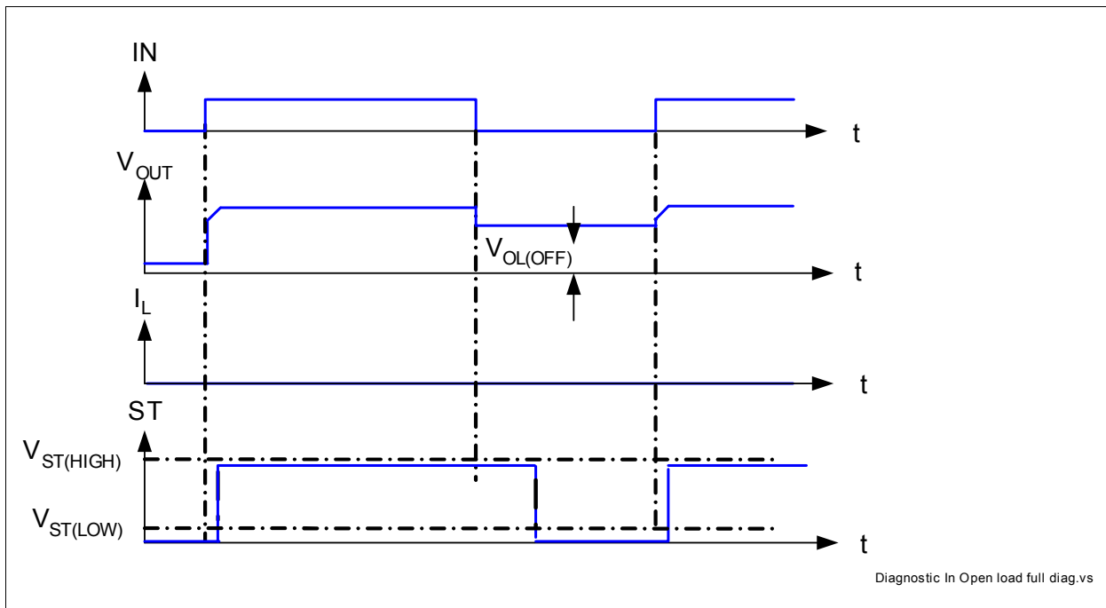
Figure 13 ST in open load condition
