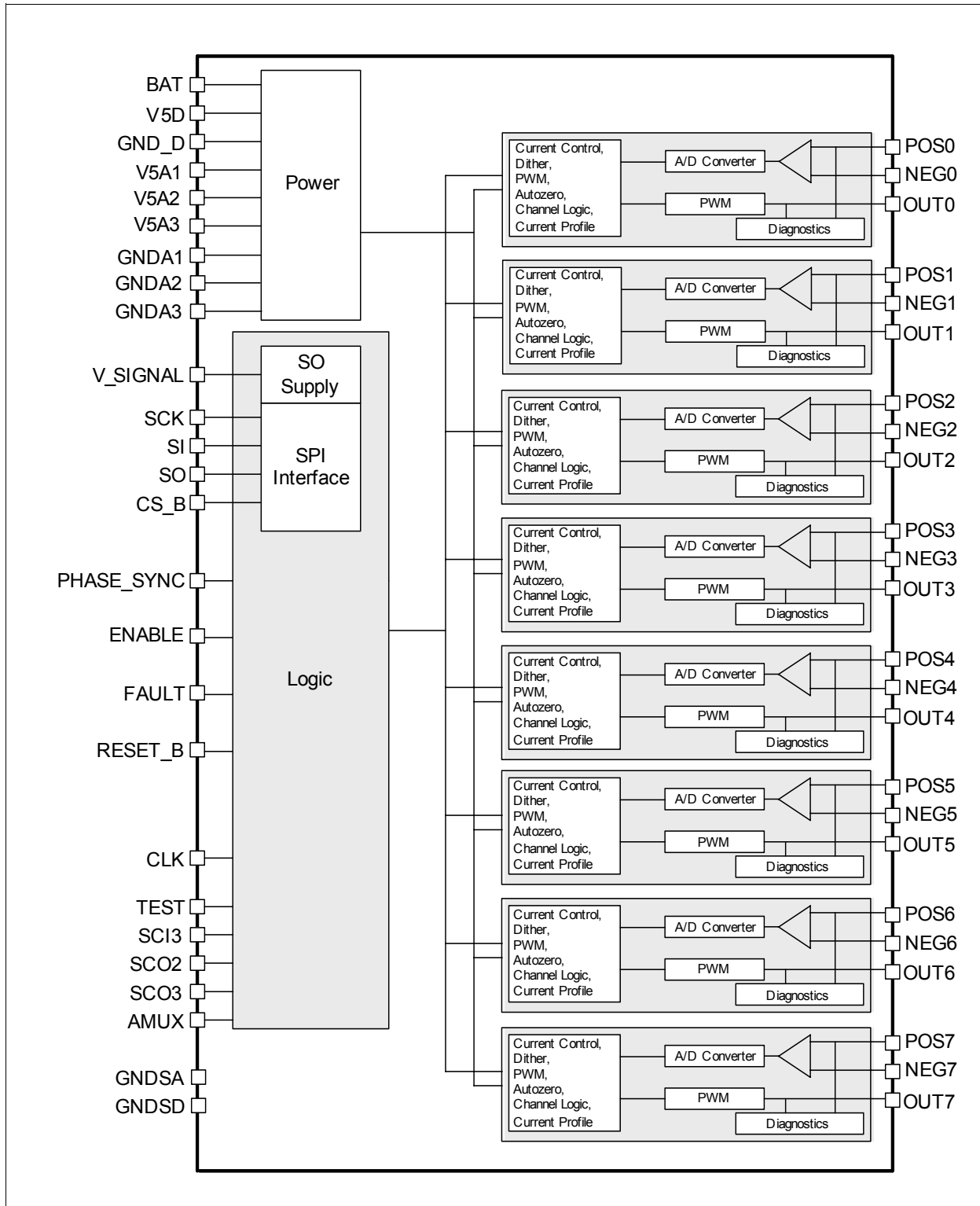
Figure 5 Block Diagram
