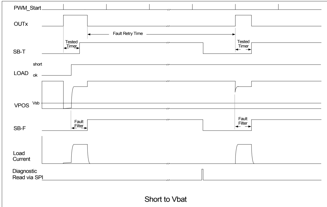
Figure 10 On-State Diagnostic Timing - Short to Vbat
