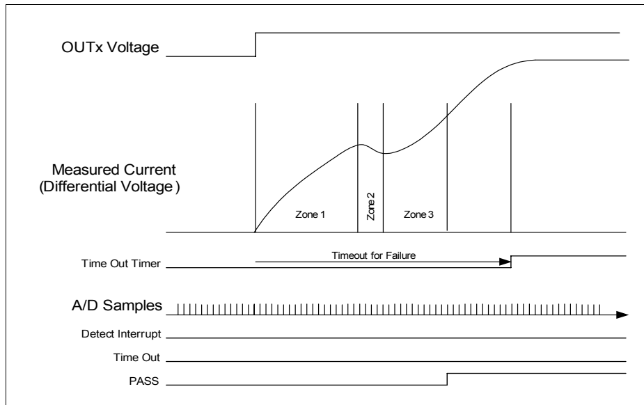
Figure 15 Current Profile Diagram - Waveform Showing Valve Movement
