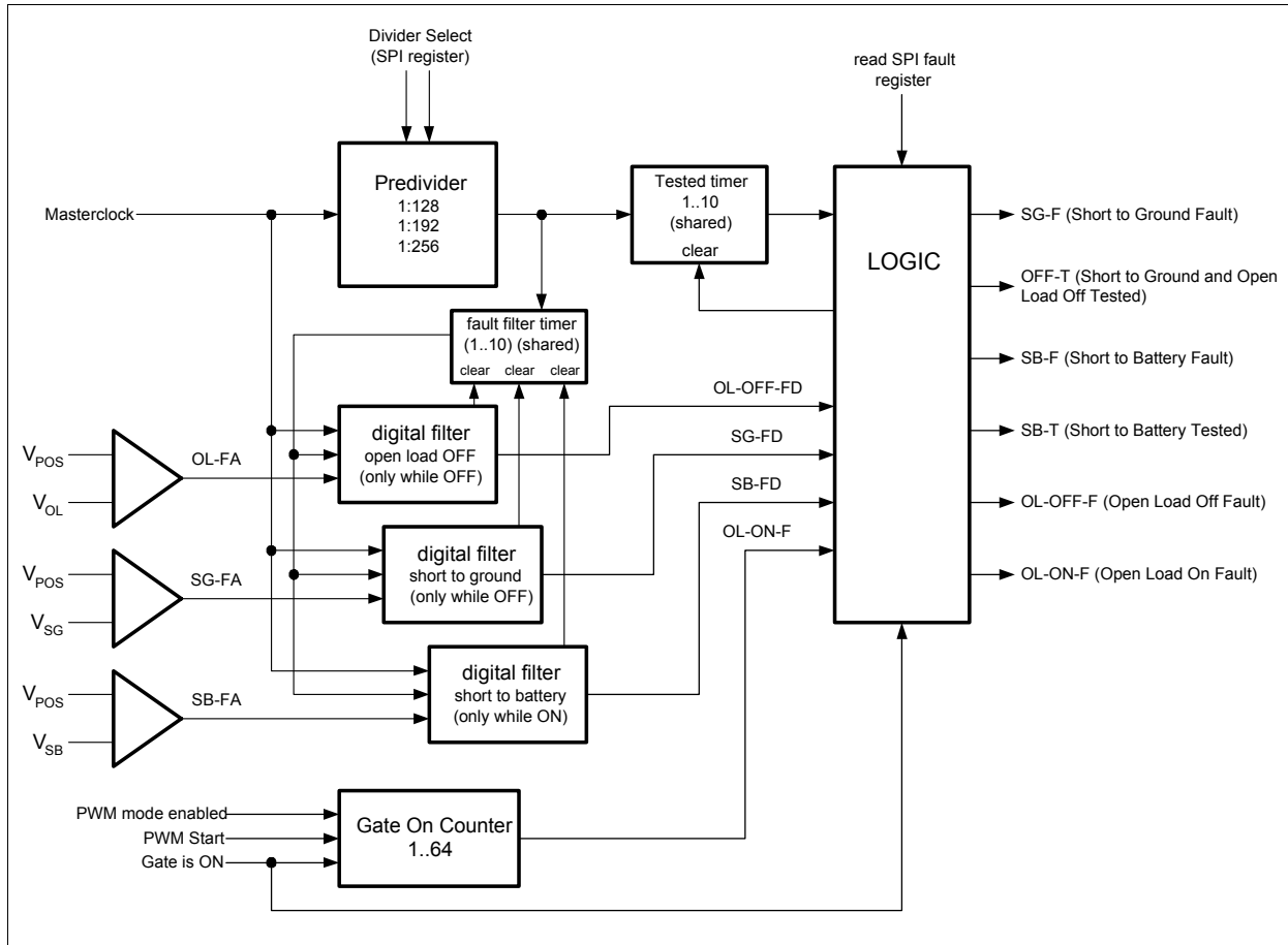
Figure 9 Diagnostic Block Diagram
