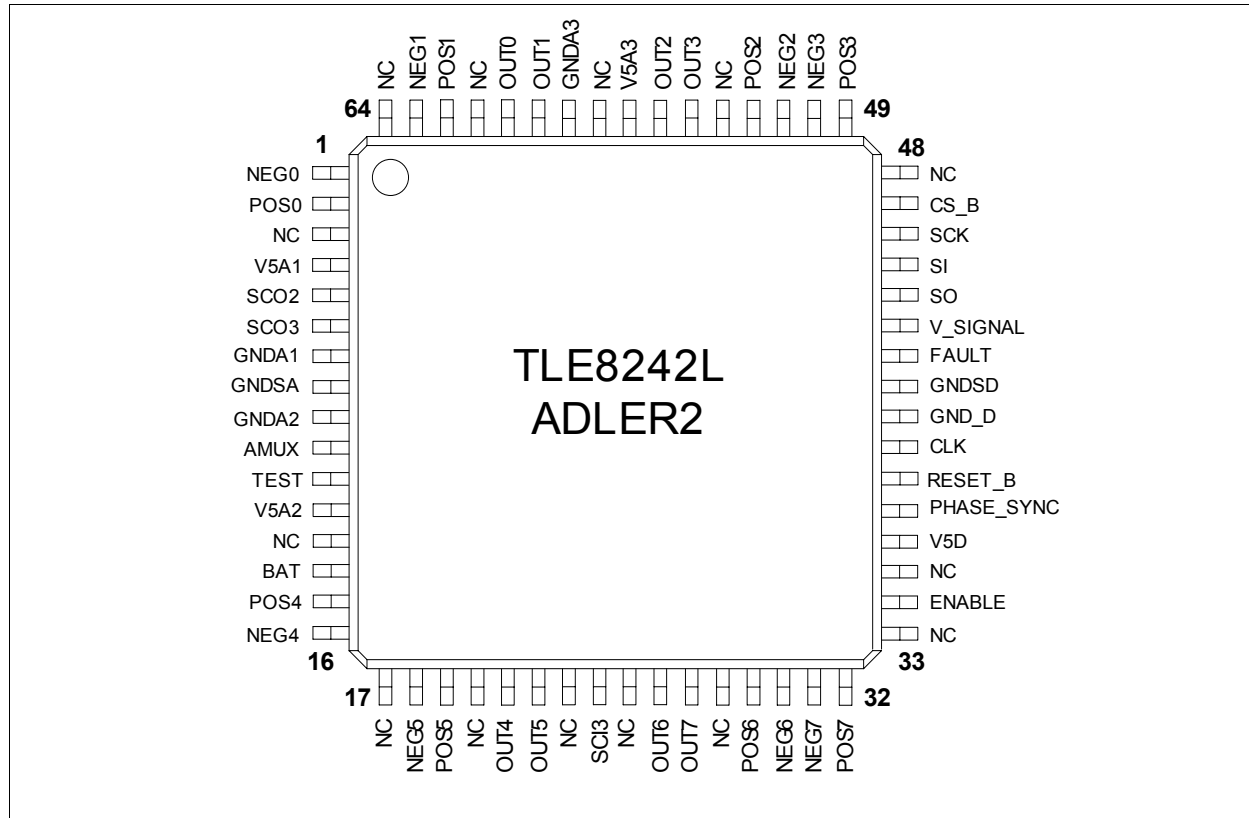
Figure 6 Pin Configuration
