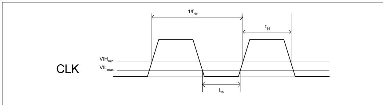
Figure 7 CLK Timing Diagram
