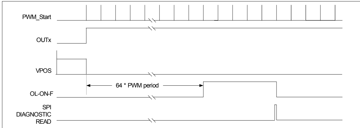
Figure 11 Open - On
