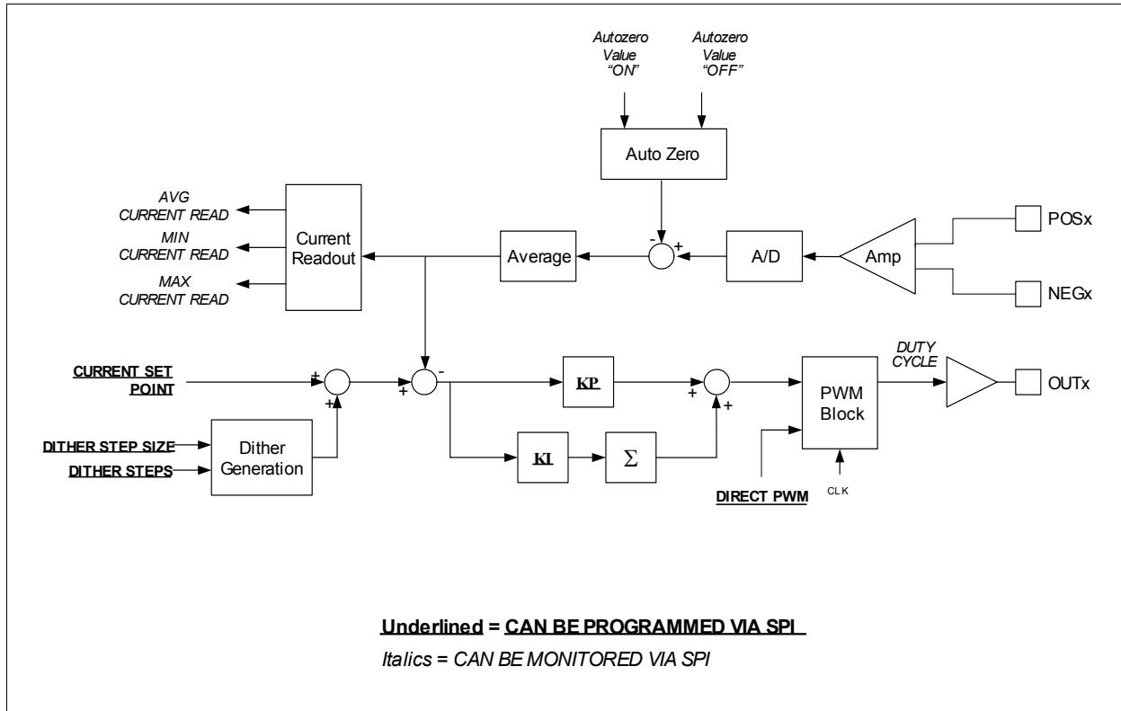
Figure 3 Control Loop - Simplified Diagram
