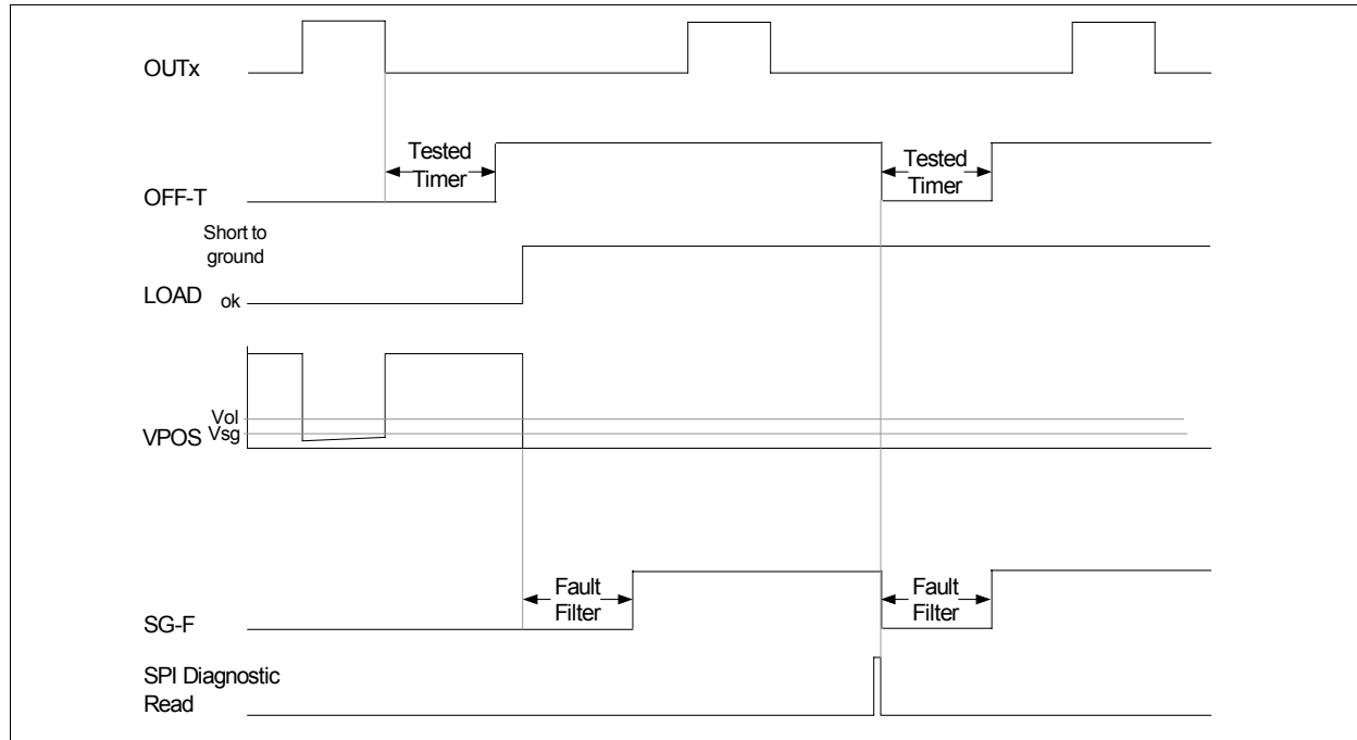
Figure 14 Off-State Diagnostics Timing Diagram - short to ground
