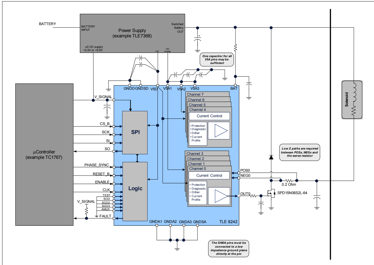
Figure 20 Application Diagram
