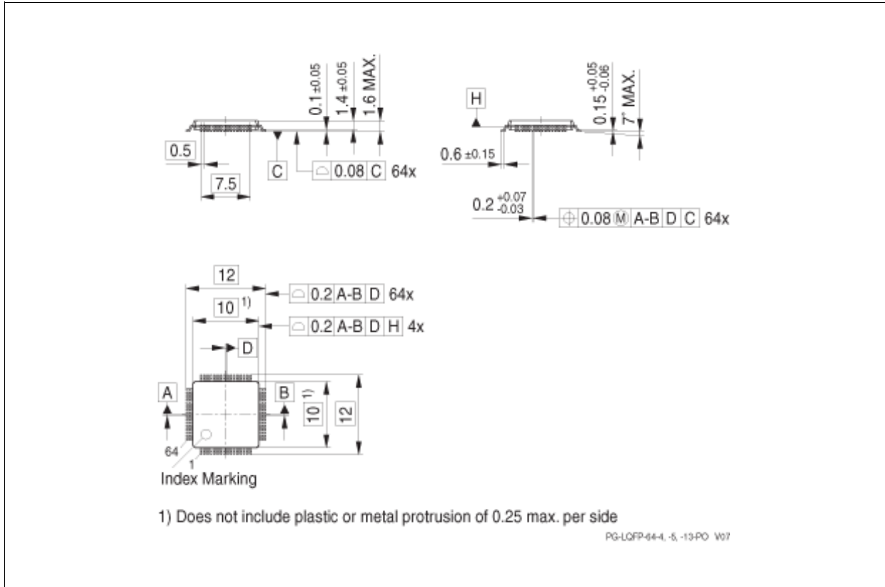
Figure 21 PG-LQFP-64
