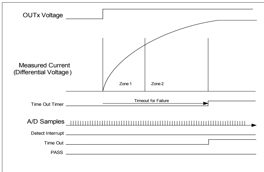
Figure 17 Current Profile Diagram - Time Out Failure
