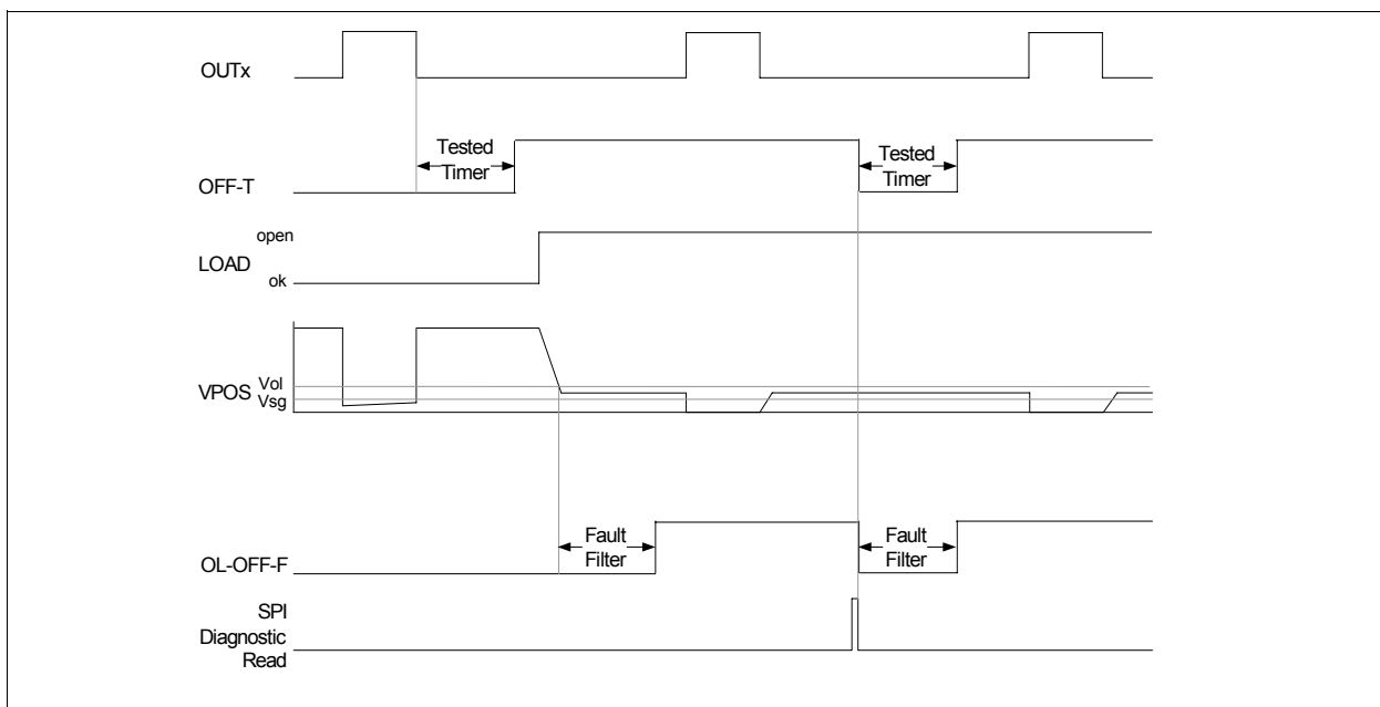
Figure 13 Off-State Diagnostics Timing Diagram - open
