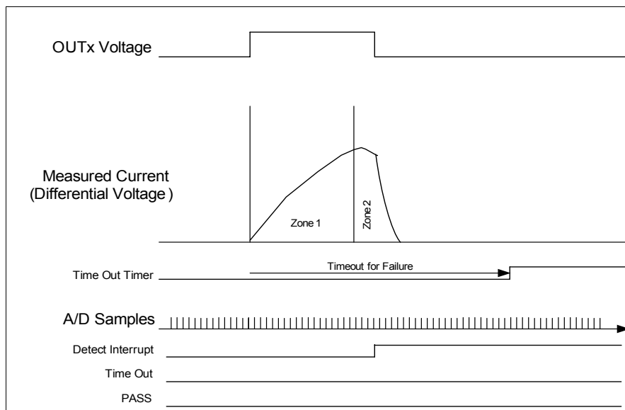
Figure 18 Current Profile Diagram - Detection Interrupted Failure
