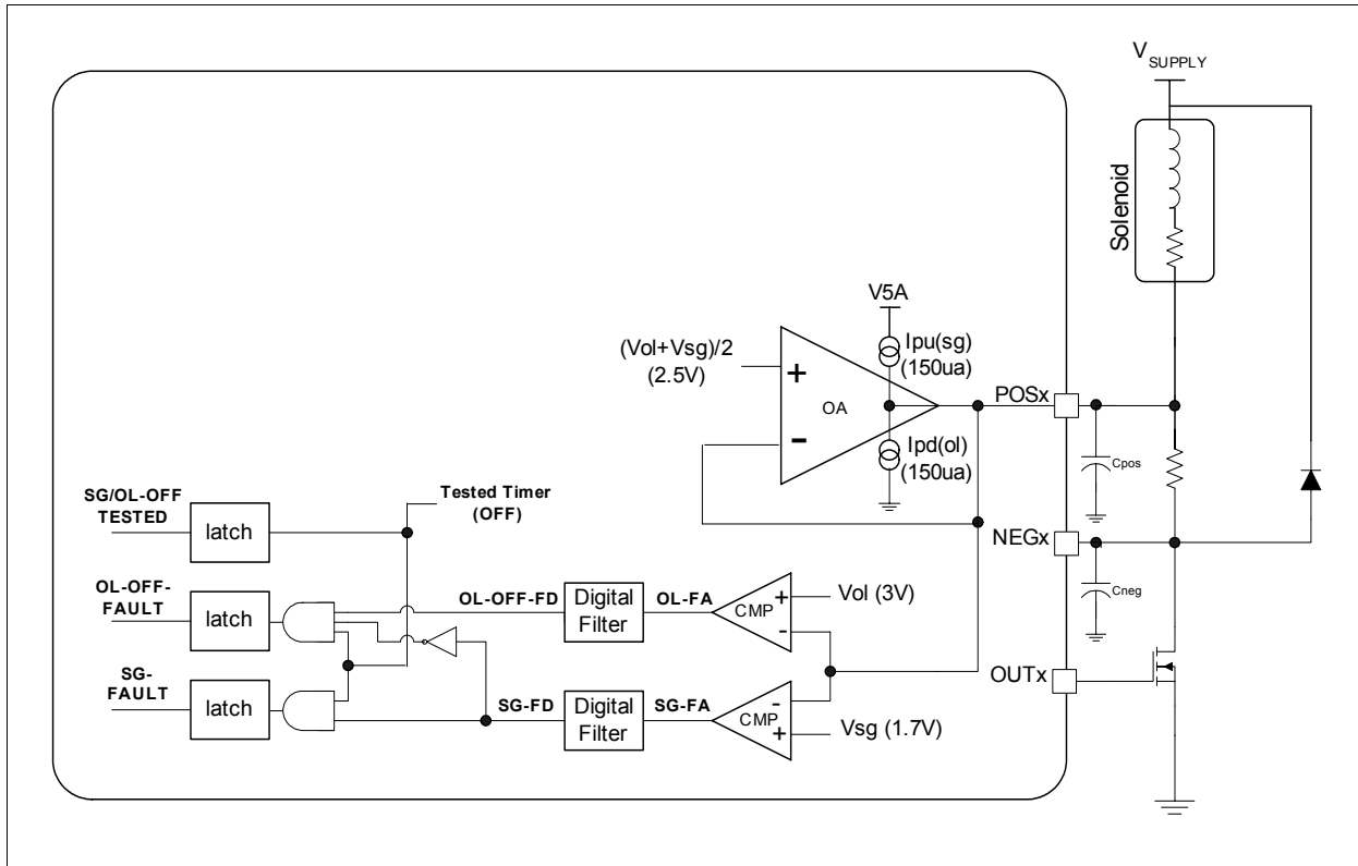
Figure 12 Off-State Diagnostics
