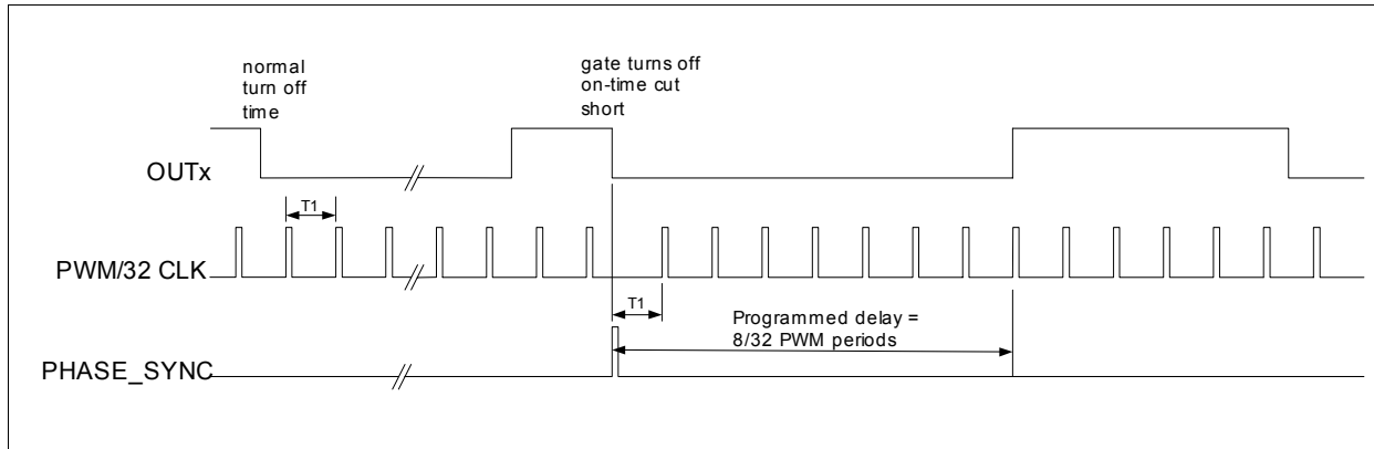
Figure 8 Phase Synchronization Diagram
