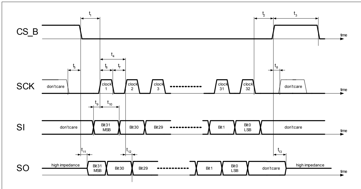
Figure 19 SPI Timing Diagram
