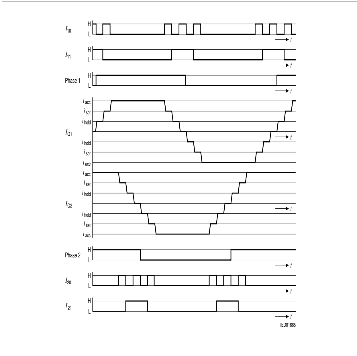
Figure 8 Mini-Step Operation
