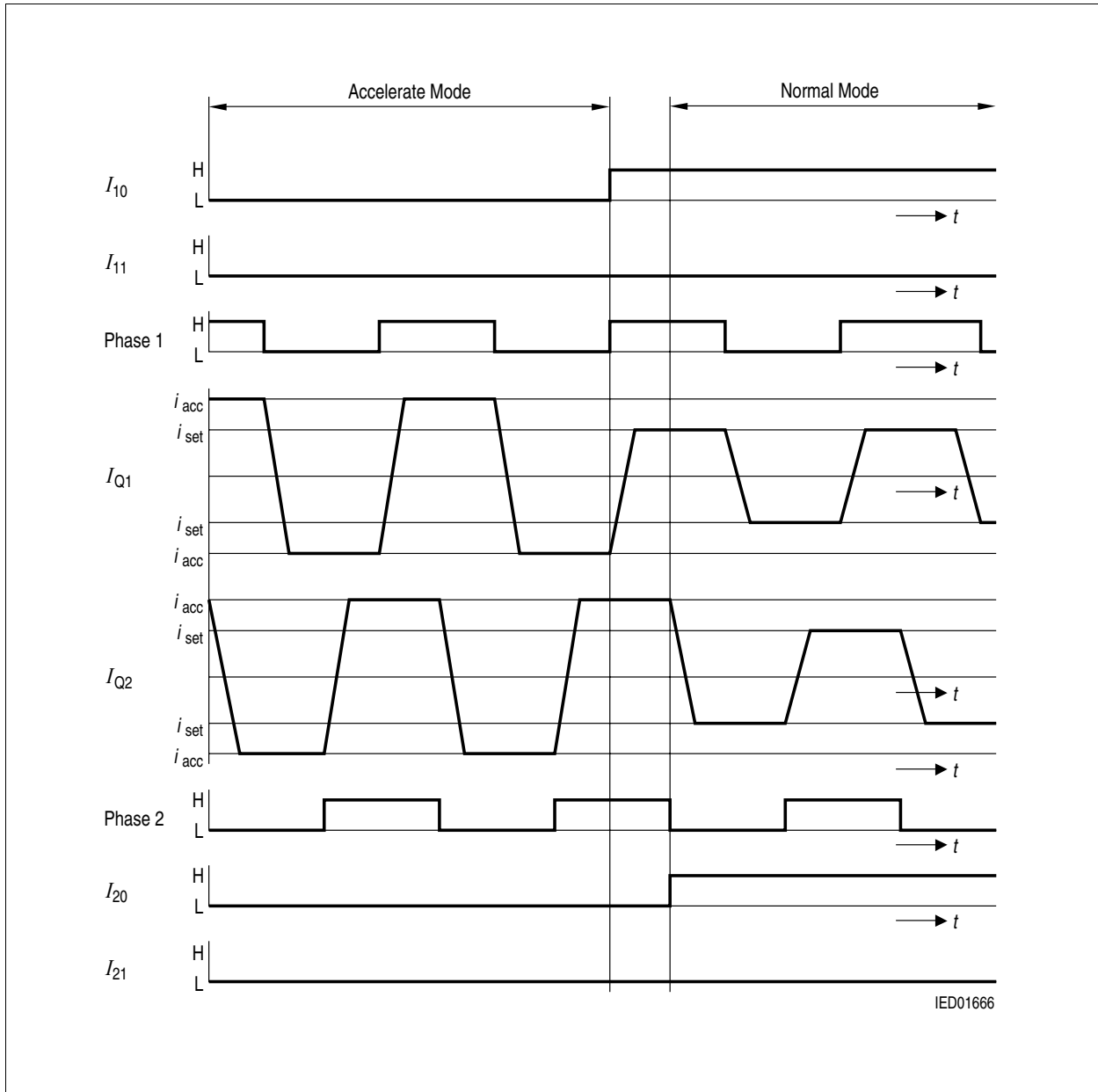
Figure 5 Full-Step Operation
