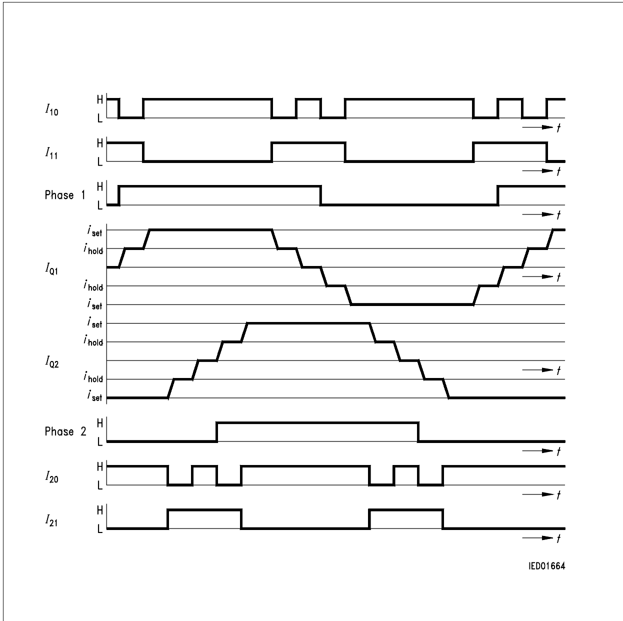
Figure 7 Quarter-Step Operation
