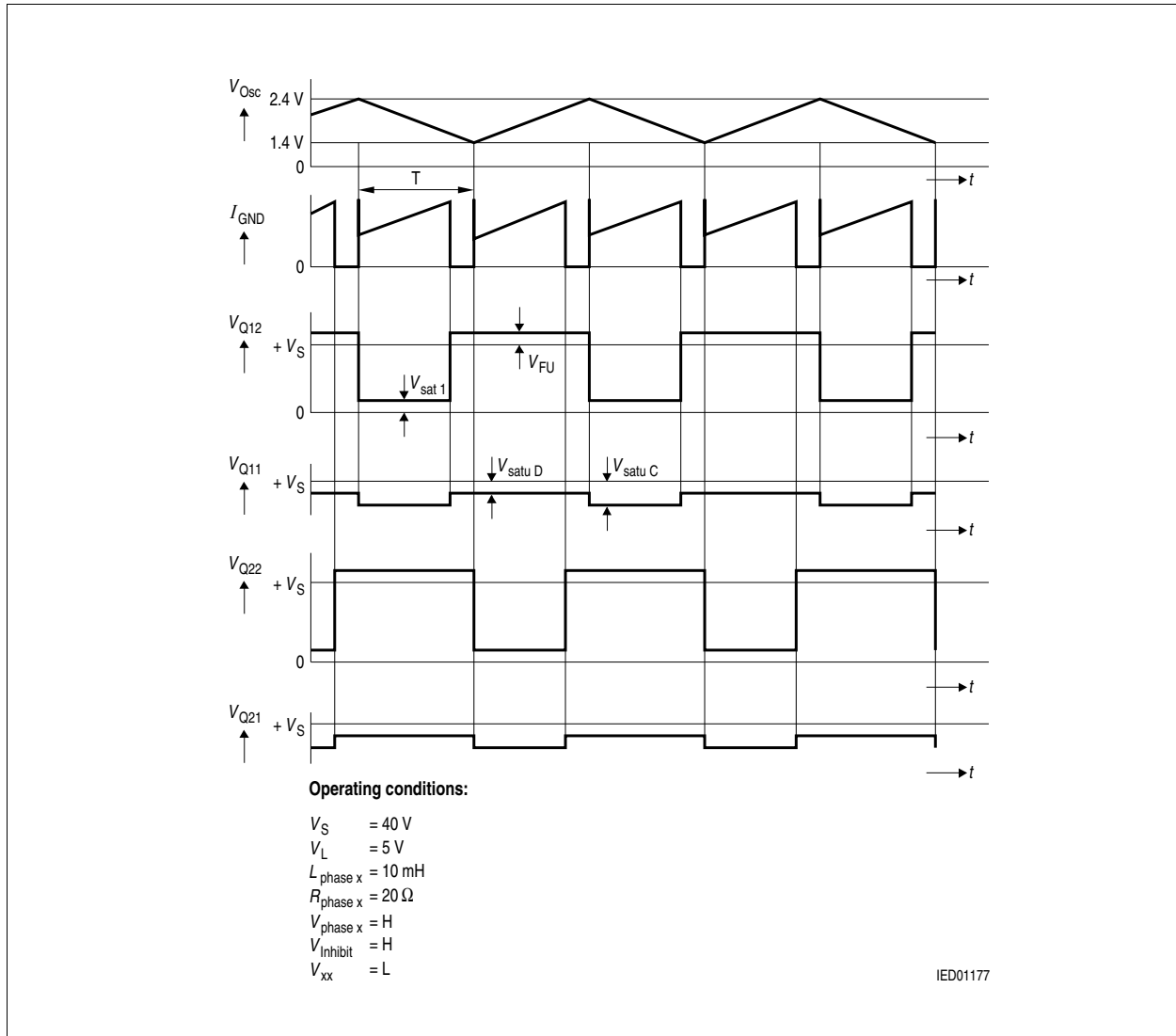
Figure 9 Current Control
