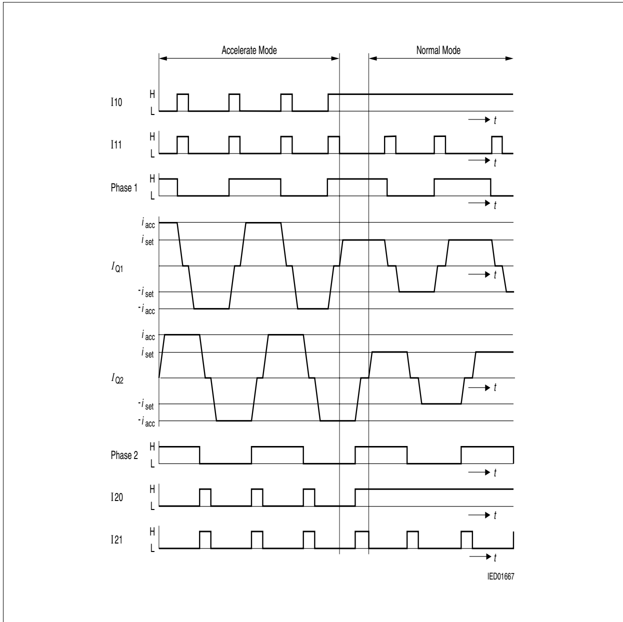
Figure 6 Half-Step Operation
