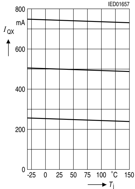
Output Current I_{QX} versus Junction Temperature T_j
