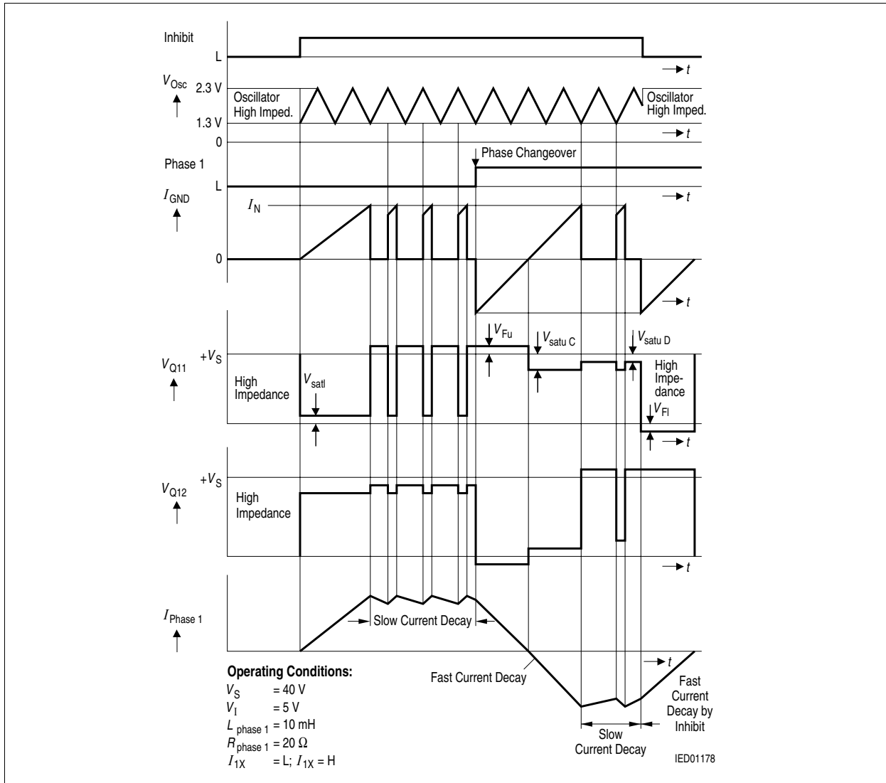
Figure 10 Phase Reversal and Inhibit
