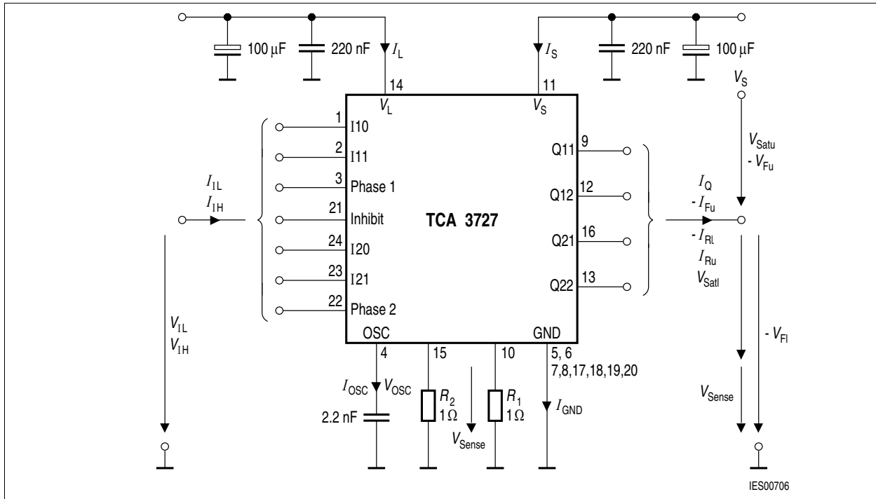
Figure 3 Test Circuit
