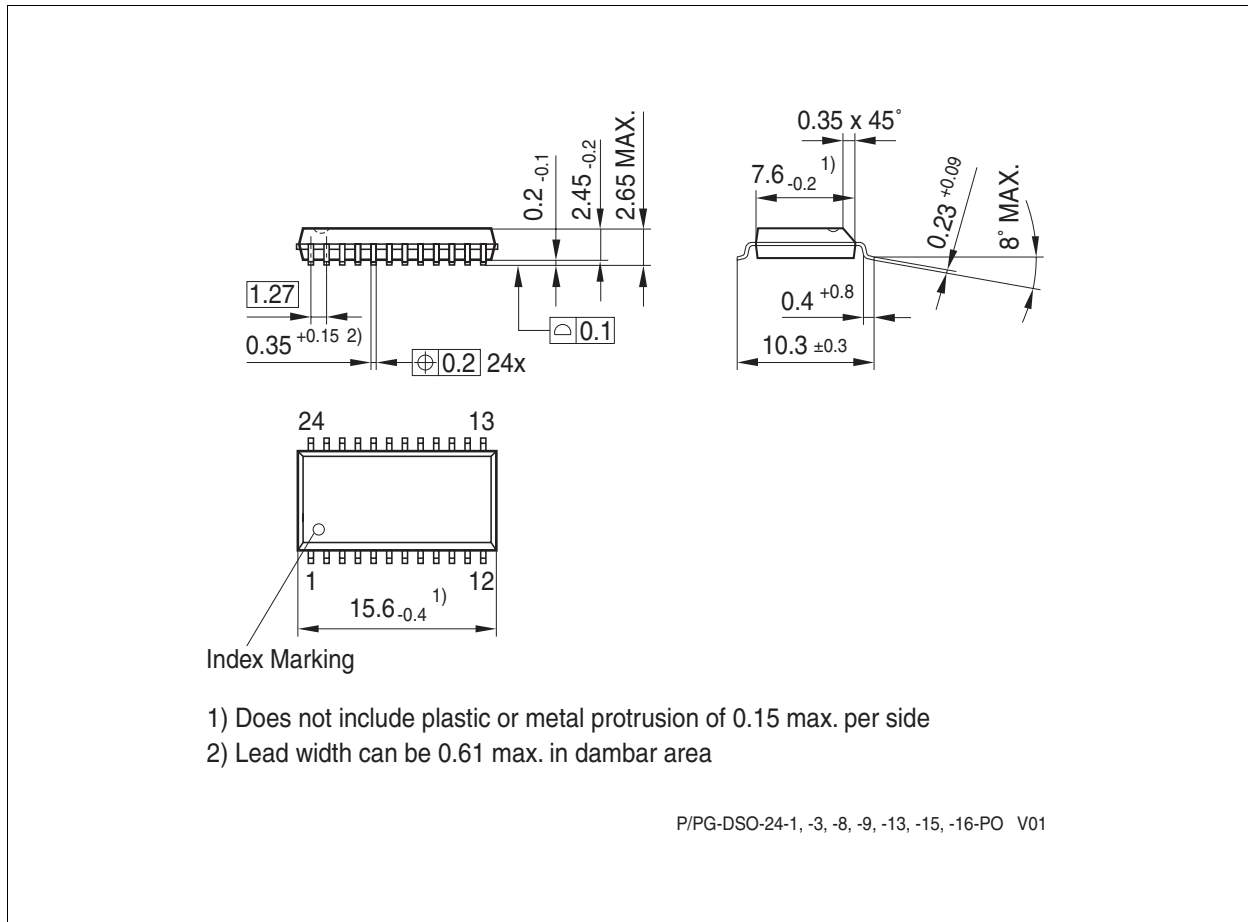
Figure 13 PG-DSO-24-13
