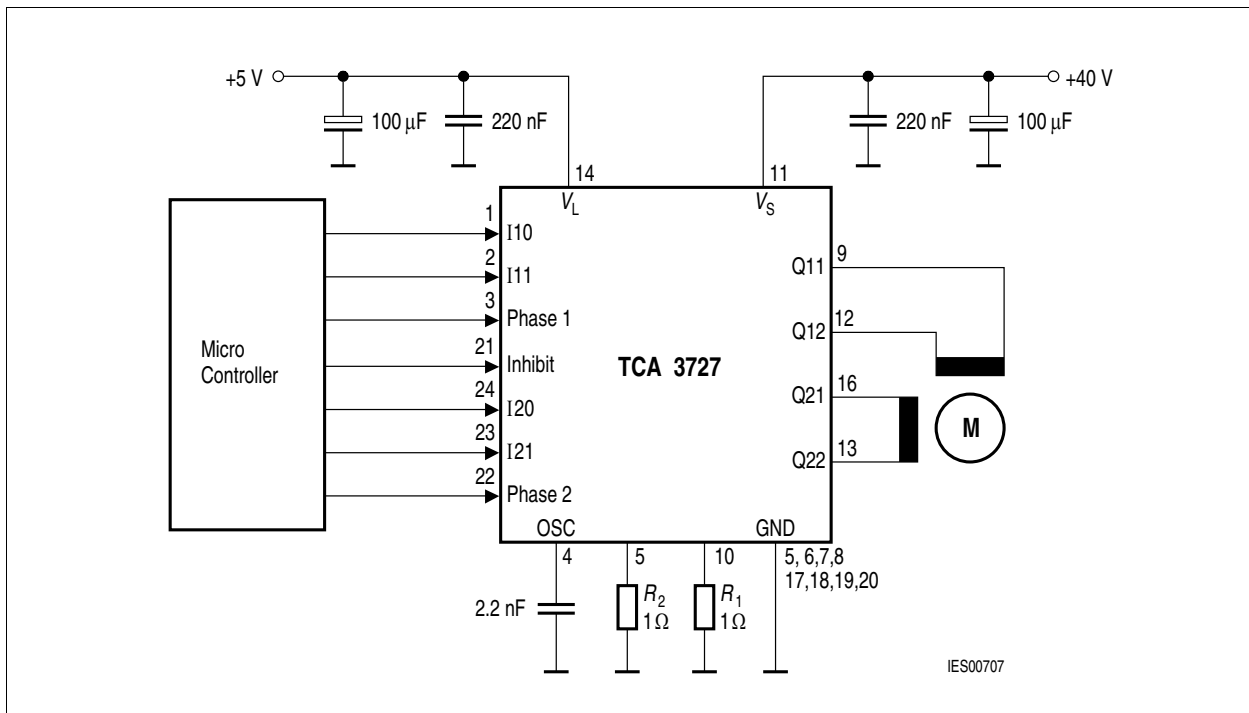
Figure 4 Application Circuit
