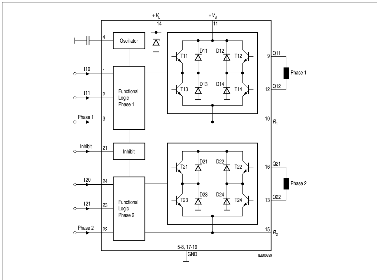
Figure 2 Block Diagram TCA 3727G
