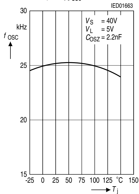
Oscillator Frequency f_{OSC} versus Junction Temperature T_j
