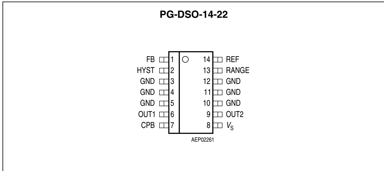
Figure 1 Pin Configuration (top view)
