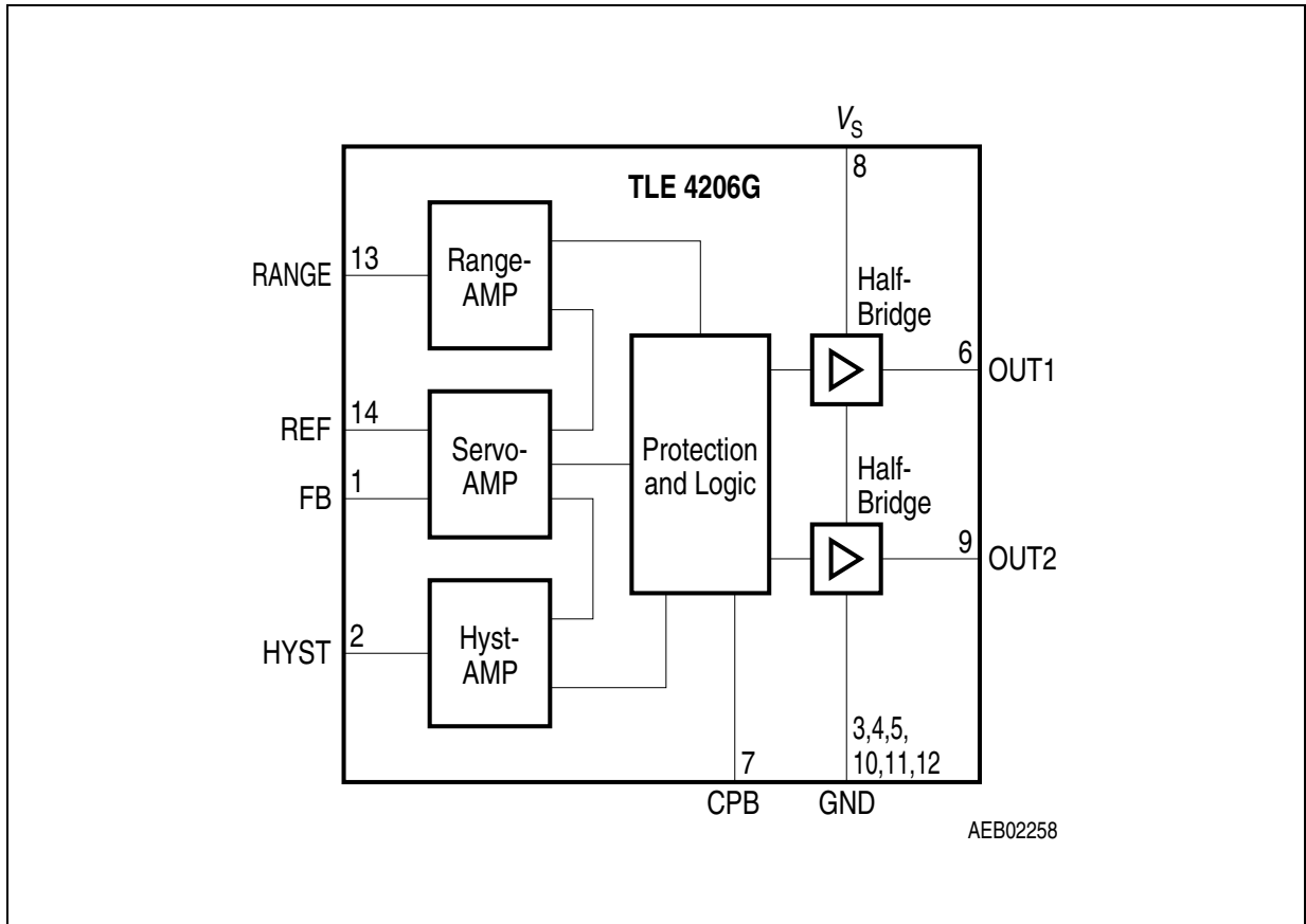
Figure 2 Block Diagram
