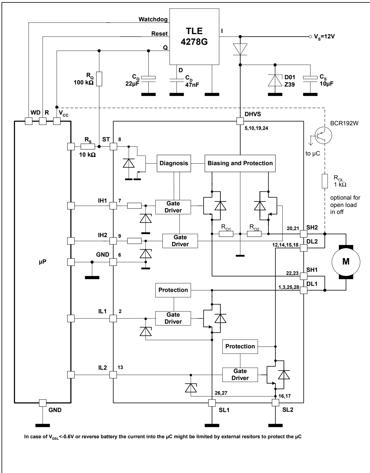
Figure 4 Application Circuit
