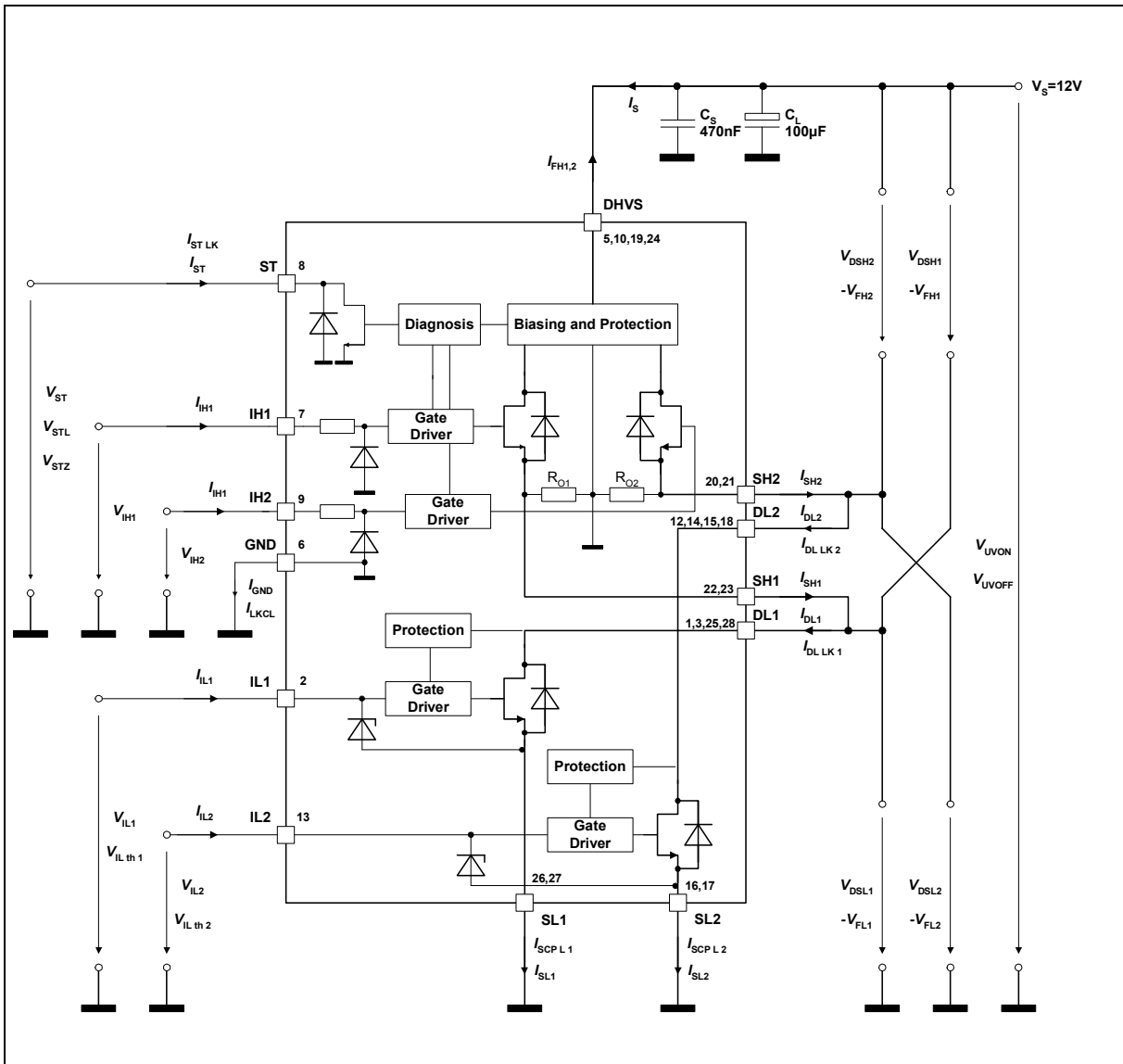
Figure 3 Test Circuit
