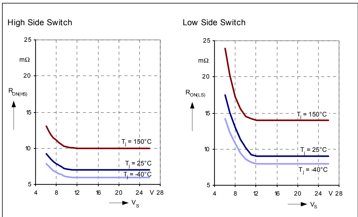
Figure 6 Typical On State Resistance vs. Supply Voltage
