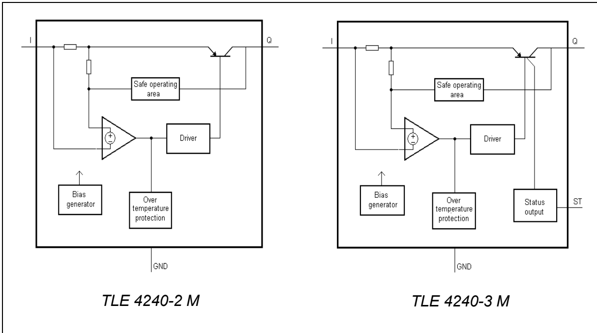
Figure 2 Block Diagram
