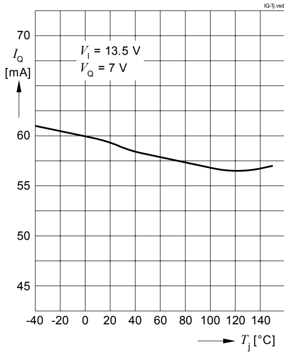
Output Current I_Q vs. Junction Temperature T_j
