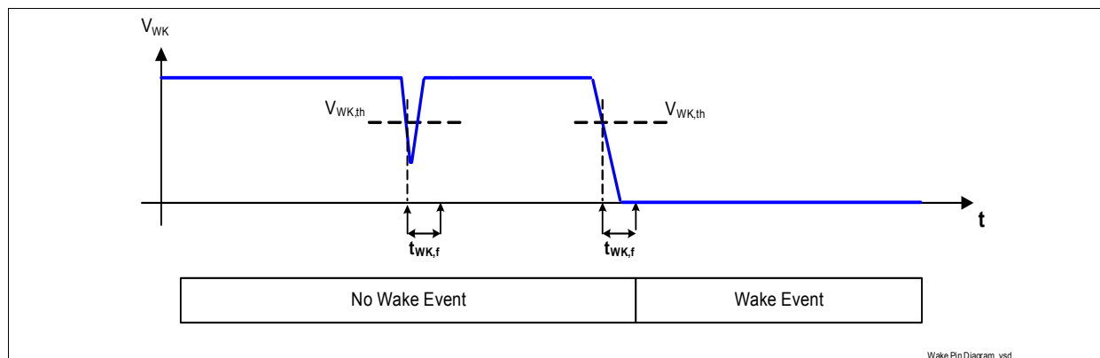
Figure 17 Wake-up Timing
