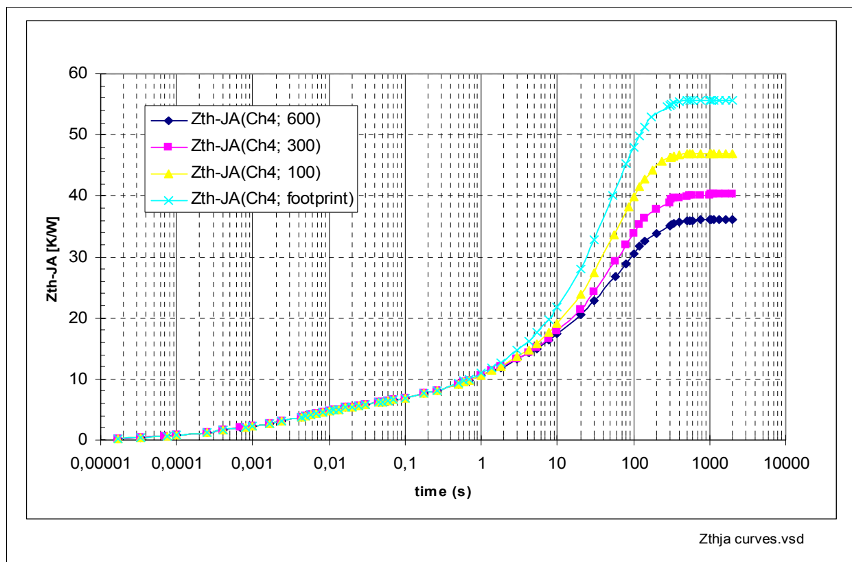
Figure 44 ZthJA Curve, Function of Cooling Area
