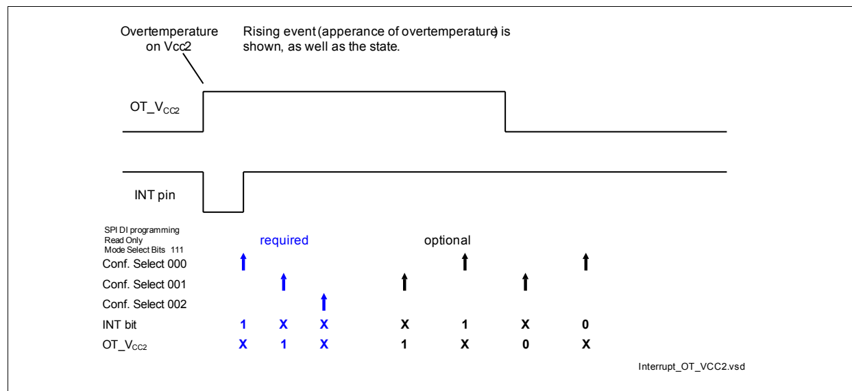
Figure 29 Interrupt Vcc2 Over Temperature.
