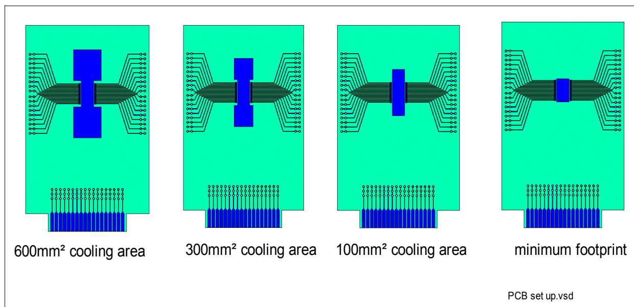
Figure 45 Board Set-up
