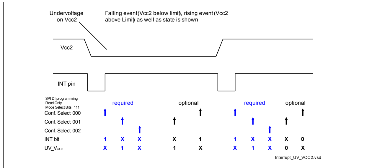
Figure 28 Interrupt Vcc2 under-voltage.
