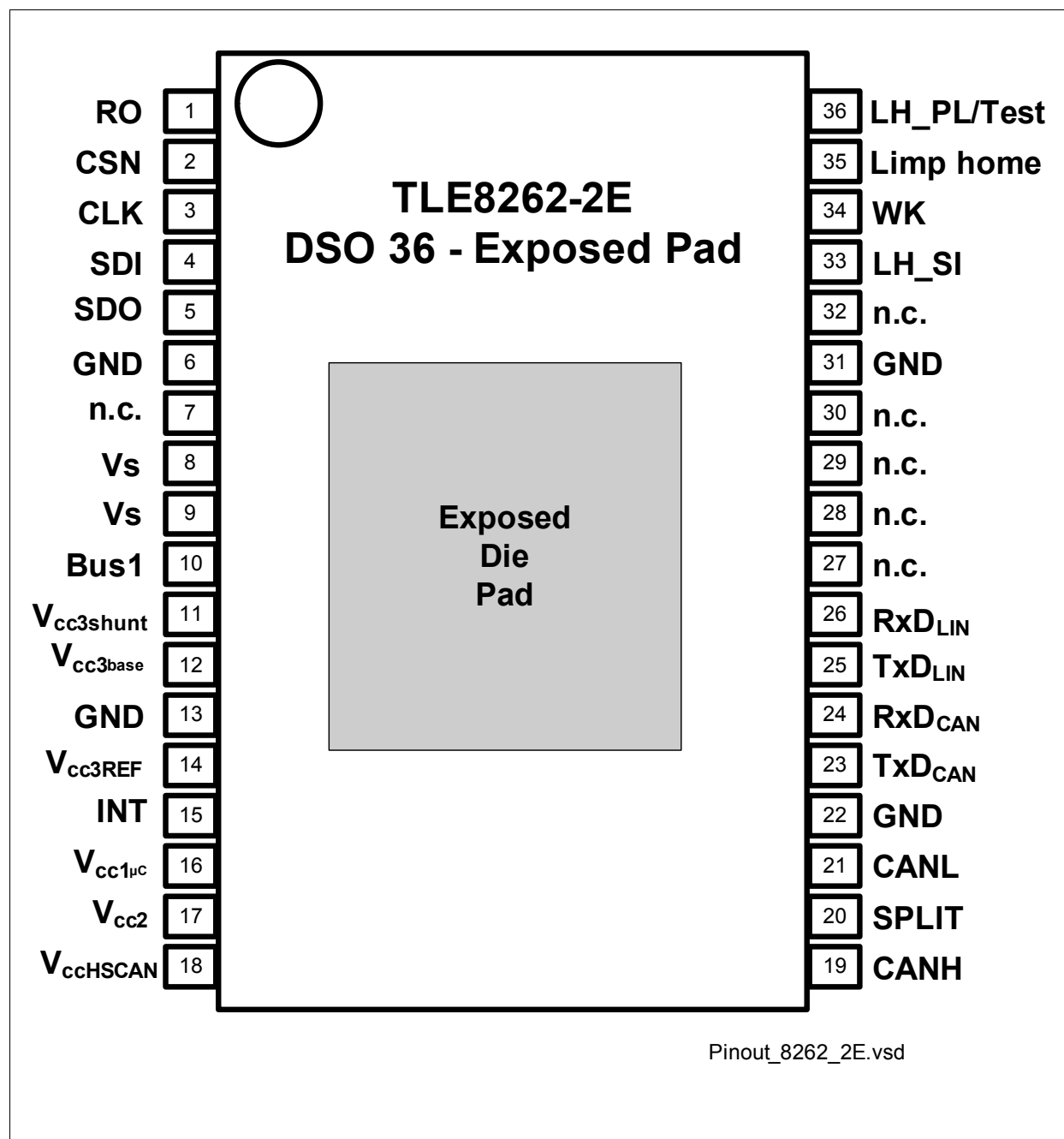
Figure 2 Pin Configuration
