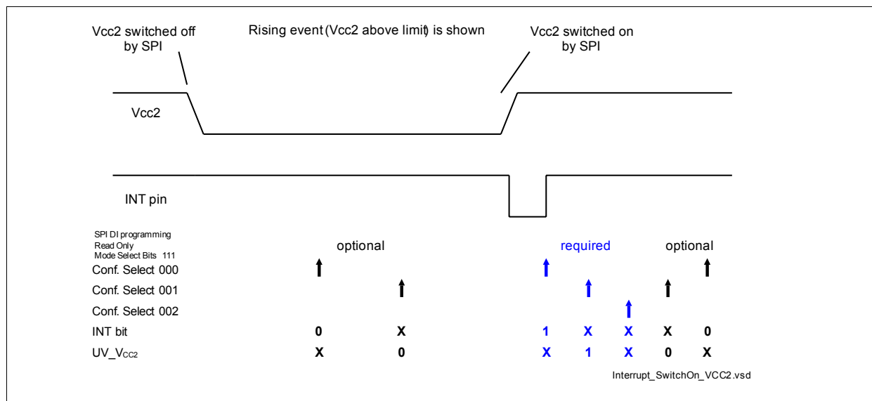
Figure 27 Interrupt Vcc2 switch-on.
