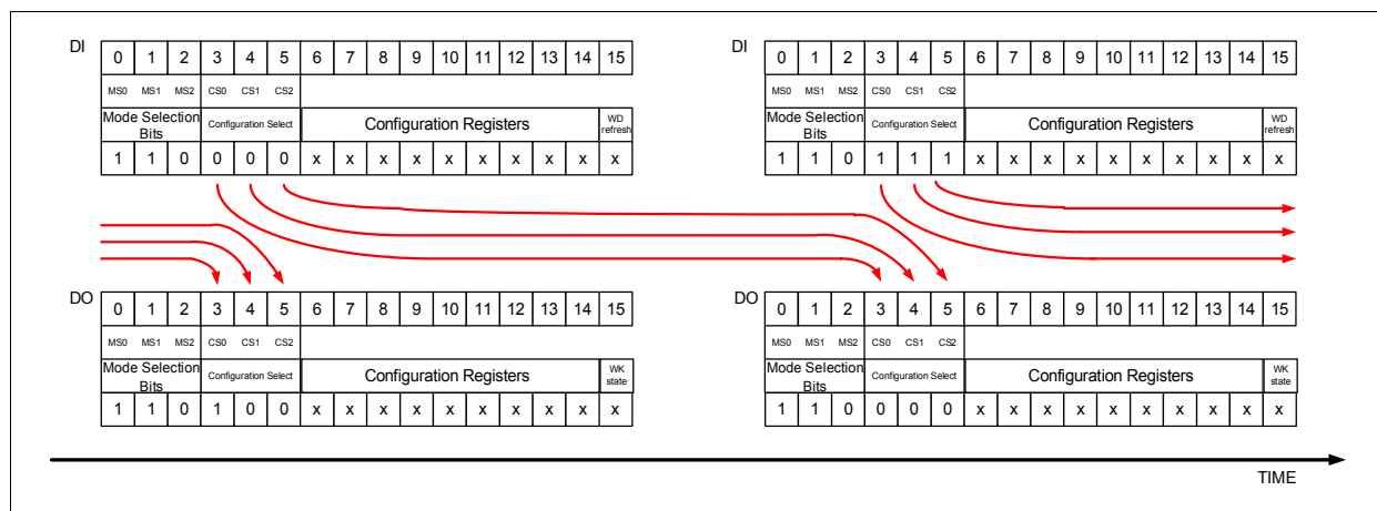
Figure 41 Write Command
