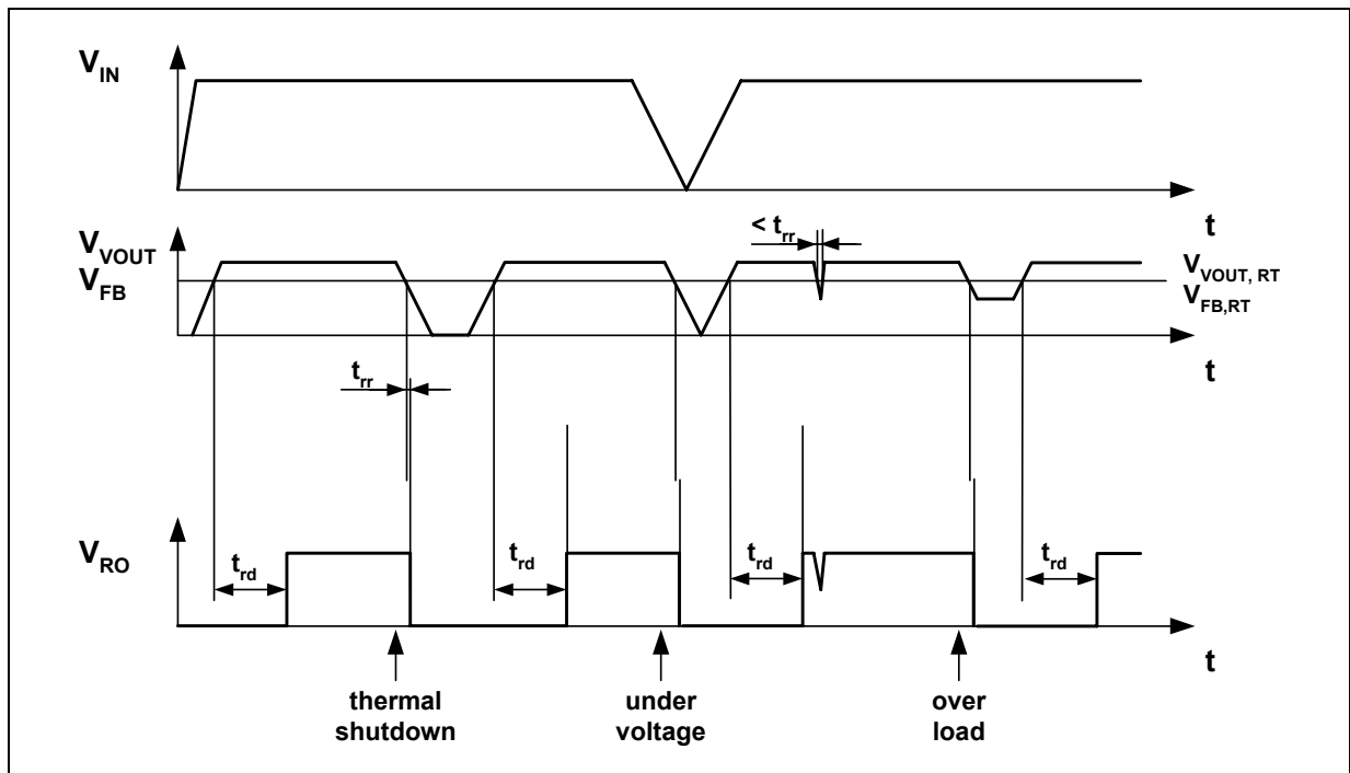
Figure 4 Reset timing
