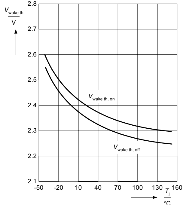
Device wake up thresholds vs. junction temperature
