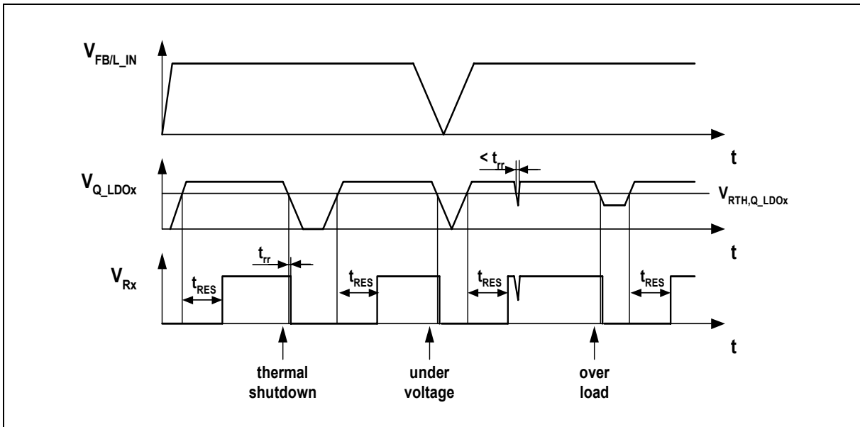
Figure 5 Undervoltage reset timing
