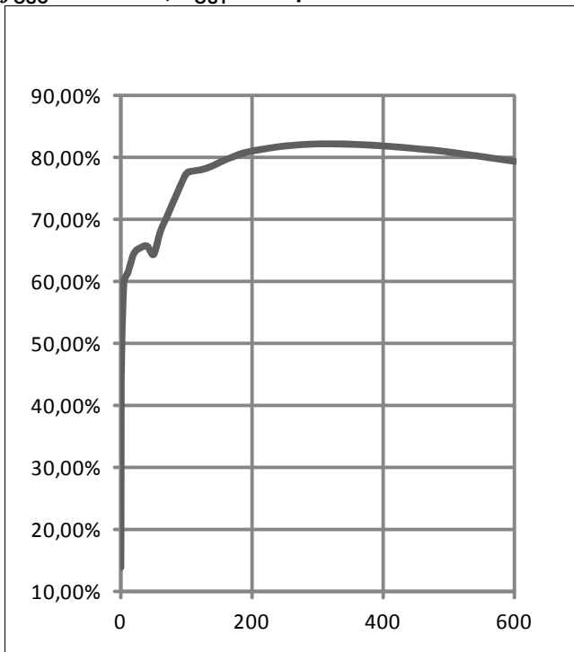
Efficiency for f_{osc} = 2.2 \text{ MHz}, L_{OUT} = 4.7 \mu\text{H}
