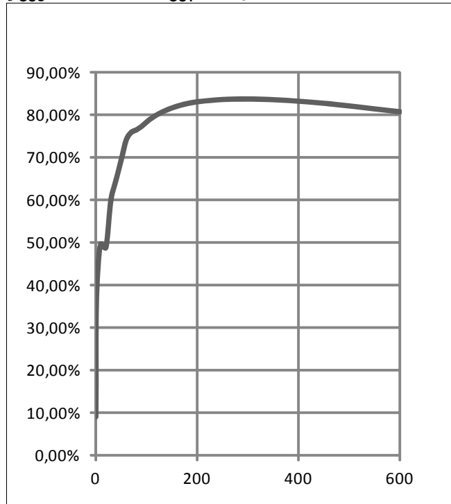
Efficiency for f_{osc} = 2.2 \text{ MHz}, L_{OUT} = 10 \mu\text{H}
