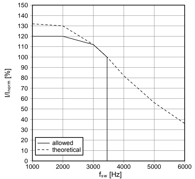
fsw - derating curve IGBT (motor) cos(phi) = 0,96 T cool medium = 40°C
